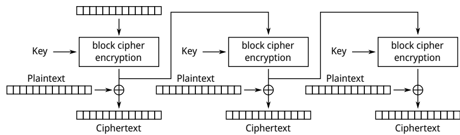
Output Feedback (OFB) mode encryption
