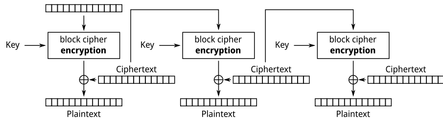
Cipher Feedback (CFB) mode decryption
