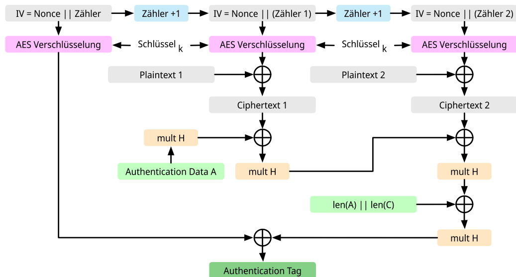
Authenticated Encryption with Additional Data (AEAD)
