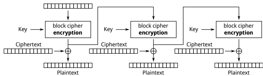
Output Feedback (OFB) mode decryption
