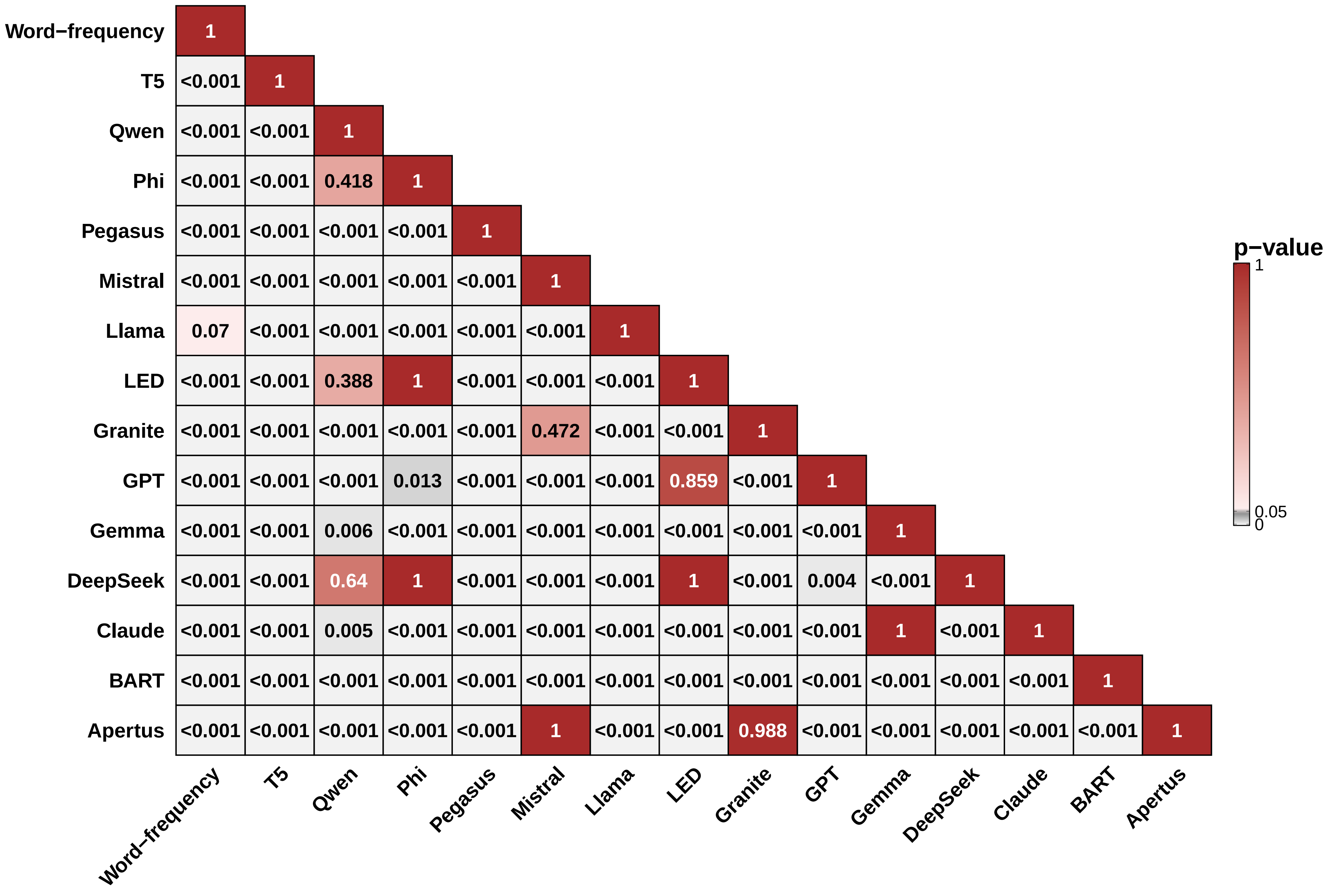
Games–Howell Post–hoc Test across Model Families
