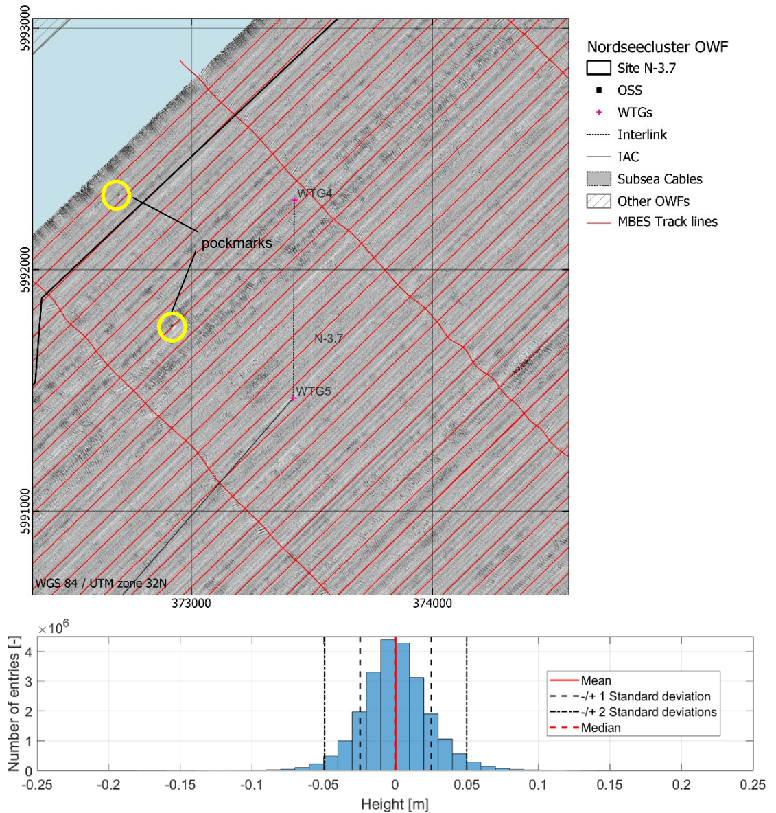
Figure 3.8 Top panel: Hillshaded view of the 2019 BSH bathymetry. The MBES track lines are marked as red lines. The locations of two pockmarks (local depressions) are marked with the yellow circles. Bottom panel: Distribution of bed forms/ undulations/ seabed roughness heights in the 2019 BSH bathymetry.
