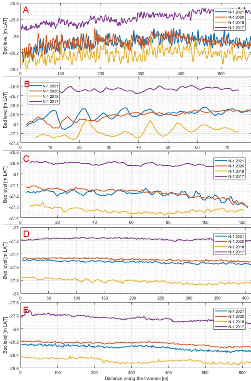
Figure 3.14 Measured bed levels along five transects in Nordsee One OWF. The location of the transects is marked in Figure 3.13. No corrections on vertical levels have been applied on the surveys.
