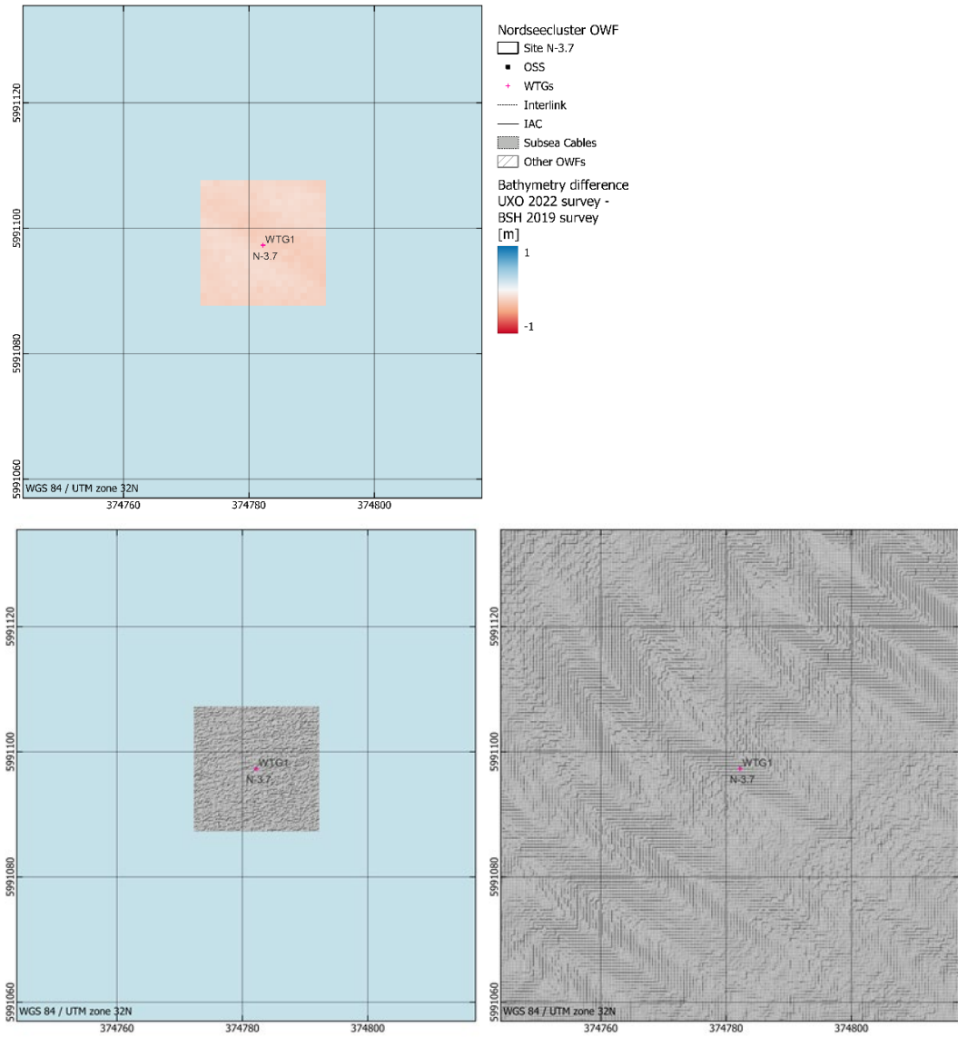
Figure 3.17 Top panel: Close up of the bathymetry differences between the 2022 UXO survey and the 2019 BSH survey close to WTG 1. The bottom left and right panels present the hillshaded view of the individual surveys over the same area.
