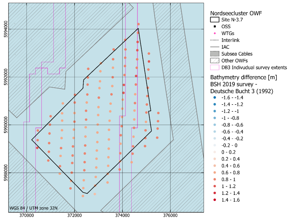
Figure 3.16 Difference between the BSH 2019 survey and the Deutsche Bucht 1992 dataset over Site N-3.7.
