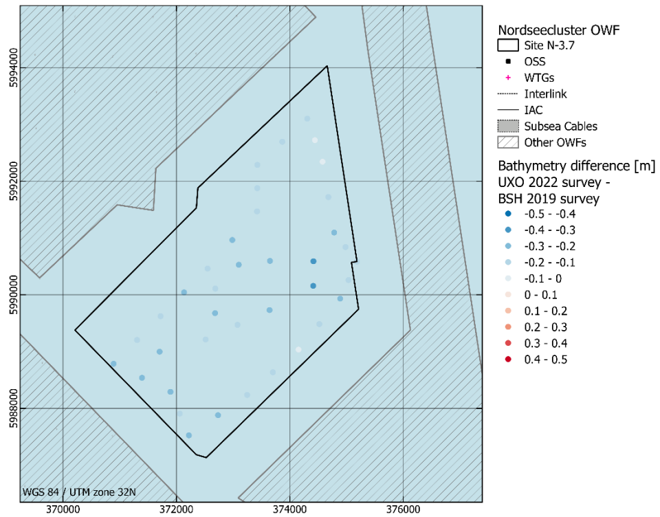
Figure 3.15 Difference between the UXO 2022 survey and the BSH 2019 survey over Site N-3.7.
