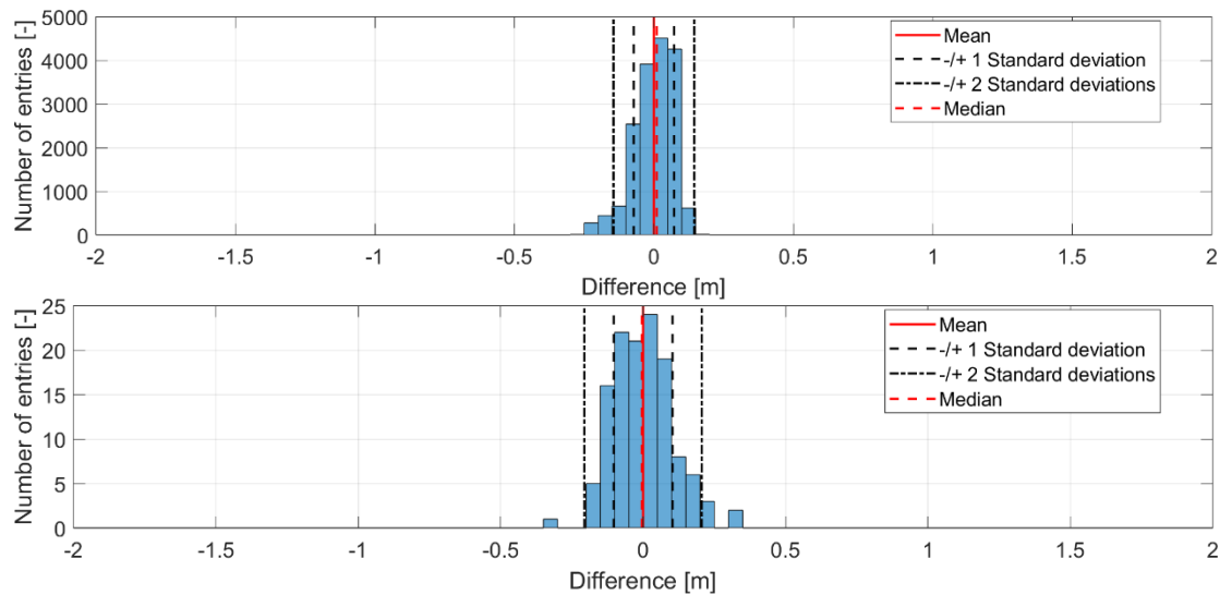
Figure 3.21 Distribution of bed level differences between the corrected 2022 UXO survey and the 2019 BSH survey (top panel) and between the BSH 2019 survey and the corrected 1992 Deutsche Bucht 3 dataset (bottom panel).
