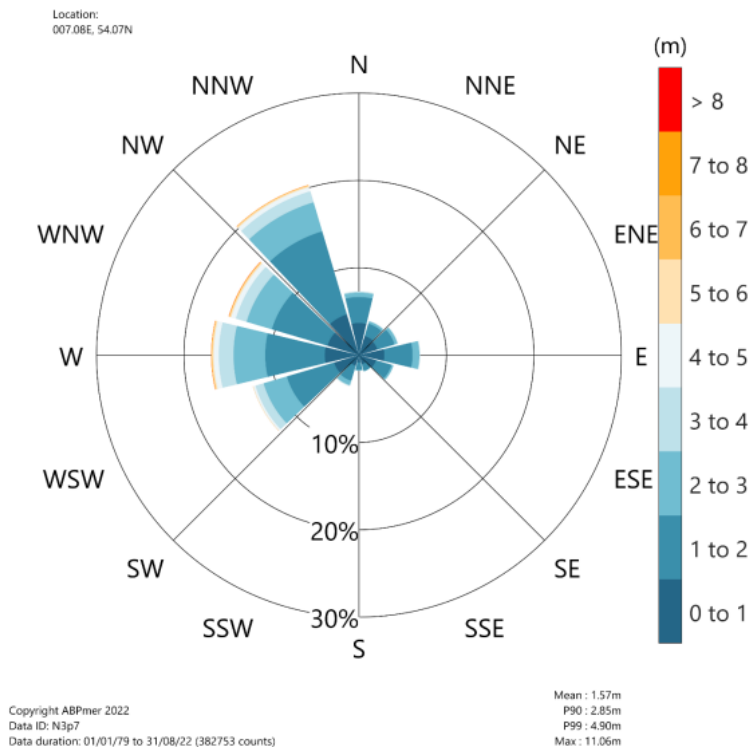
Figure 2.6 Annual significant wave height rose at location N3.7-SW (ABPmer, 2023b). Wave directions correspond to the direction the waves are coming from.
