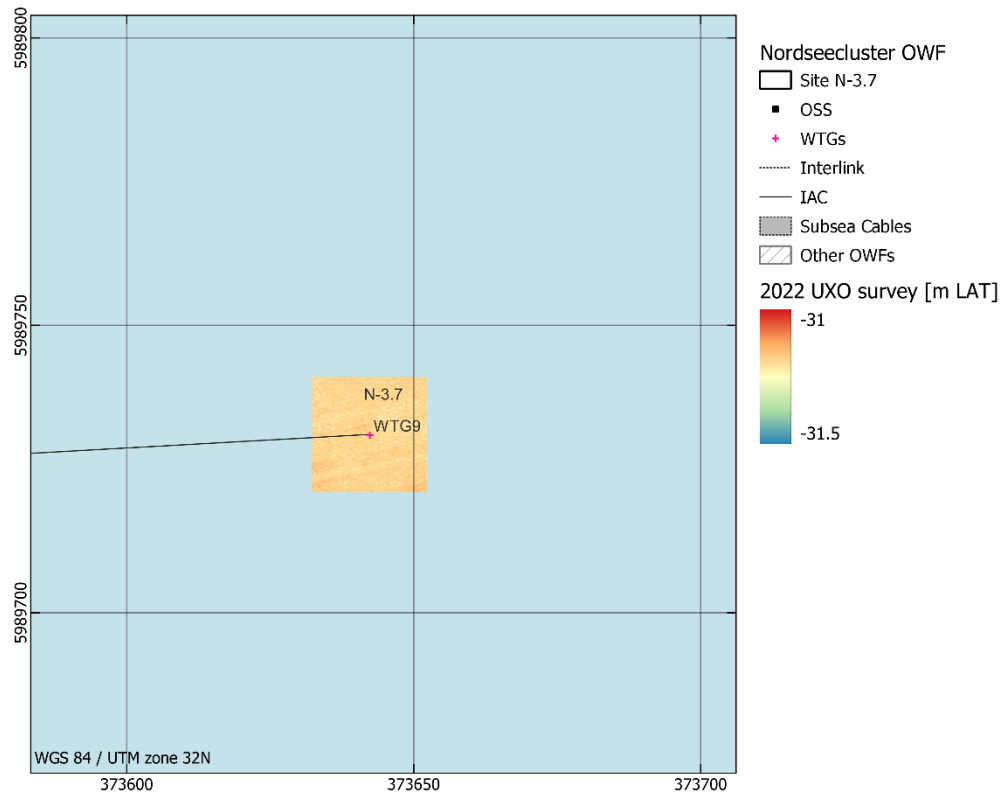
Figure 2.1 Top panel: Overview of the BSH 2019 bathymetry over Site N-3.7. The outline of Site N-3.7 is marked with a black line. Bottom panel: Close-up view of the UXO 2022 bathymetry around WTG 09.
