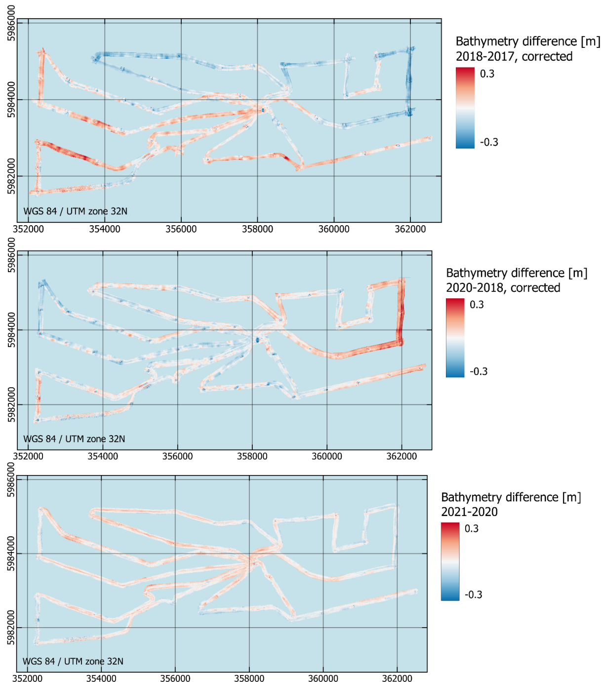
Figure 3.28 Seabed level differences between the 2017 and 2018 surveys (corrected, top panel), 2018 and 2020 surveys (corrected, middle panel) and 2020 and 2021 survey (bottom panel), over the Nordsee One OWF.
