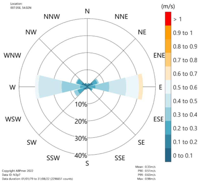
Figure 2.5 Top panel: Annual current velocity at surface (top of the water column) at FINO1. Bottom panel: Annual total depth averaged current velocity at point N3.7_HD (ABPmer, 2023b). Current directions correspond to the directions the currents are moving towards.
