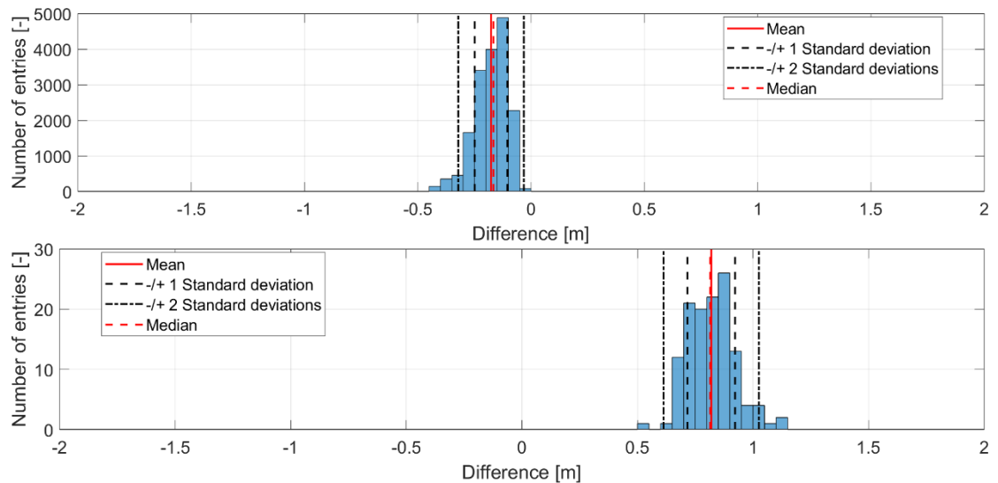
Figure 3.18 Distribution of bed level differences between the 2022 UXO survey and the 2019 BSH survey (top panel) and between the BSH 2019 survey and the 1992 Deutsche Bucht 3 dataset (bottom panel).
