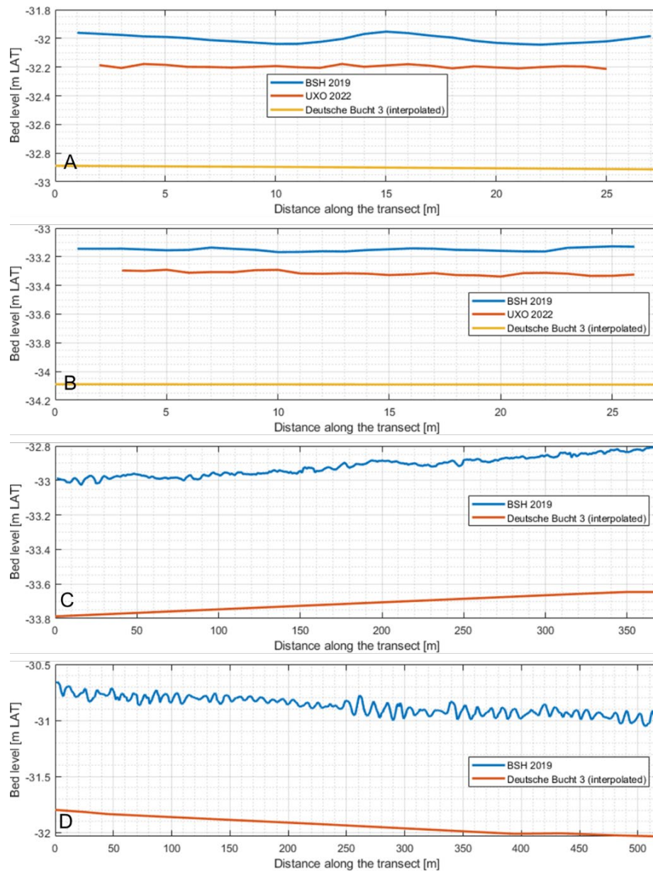
Figure 3.11 Measured bed levels along four transects in Site N-3.7. The location of the transects is presented in Figure 3.10. No corrections on vertical levels have been made on the surveys.
