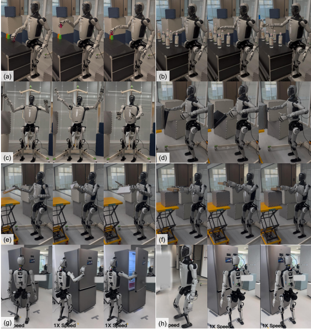
Fig. 8: Manipulation tasks. (a) grab the cup and put it onto cups, (b) take and deliver a bottle of water, (c) dance with arms but slow down the original motions while the lower body maintains balance, (d) open the oven, (e) Take the book and pass it from left hand to right hand, (f) carry a box, (g) Loco-open-fridge, (h) loco-button-pressing task.
