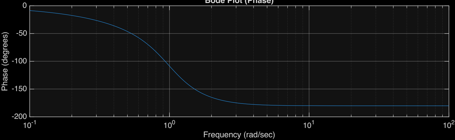
Bode Plot (Phase)
