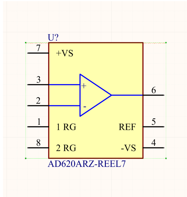
Figure 1.2. Schematic library for AD620ARZ-REEL7
