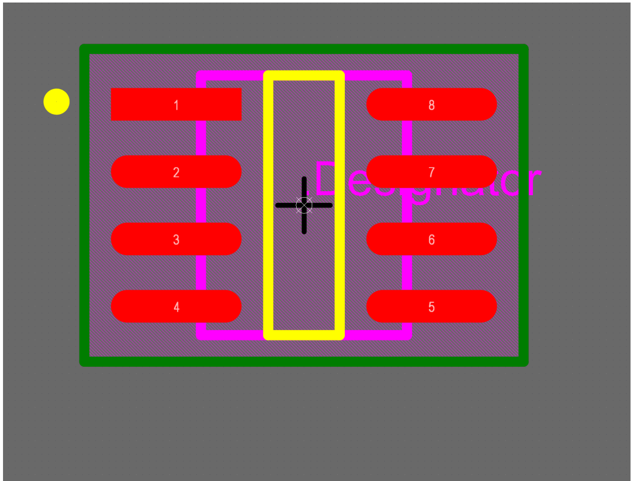
Figure 2.1. PCB library for AD620ARZ-REEL7.
