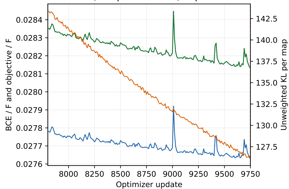
Stochastic train (10-update means) · updates 7801-9750
