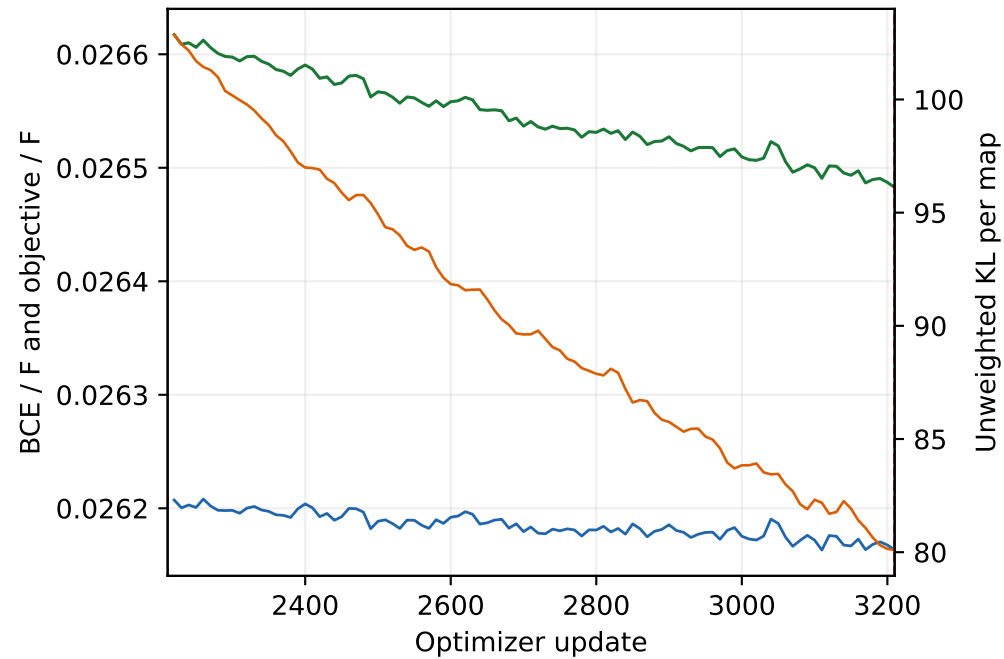
Stochastic train (10-update means) · updates 2211-3210
