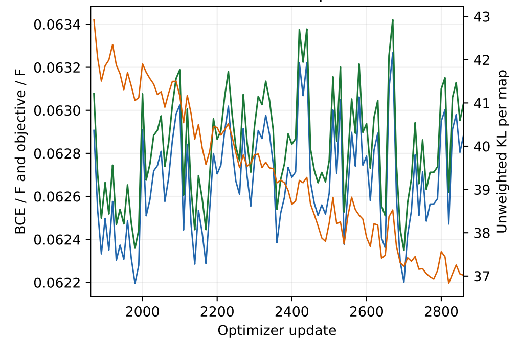
Posterior-mean validation · updates 1861-2860
