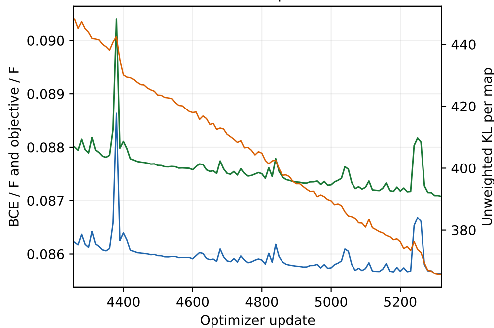
Posterior-mean train · updates 4257-5320
