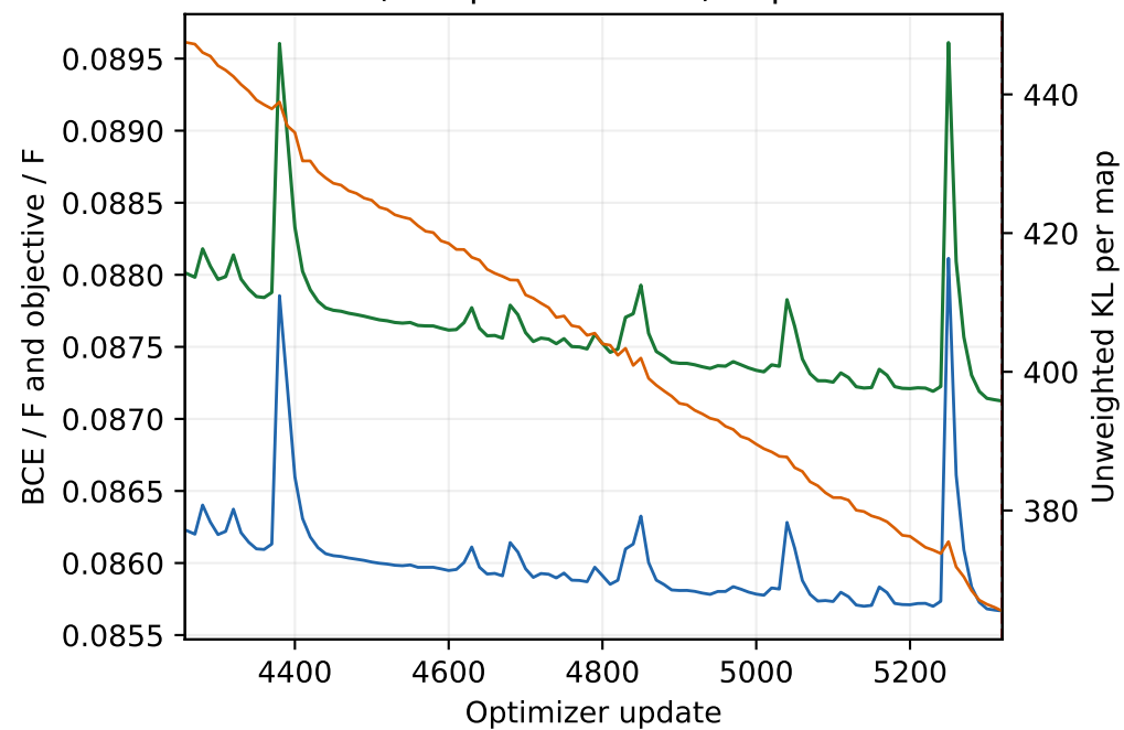
Stochastic train (10-update means) · updates 4257-5320
