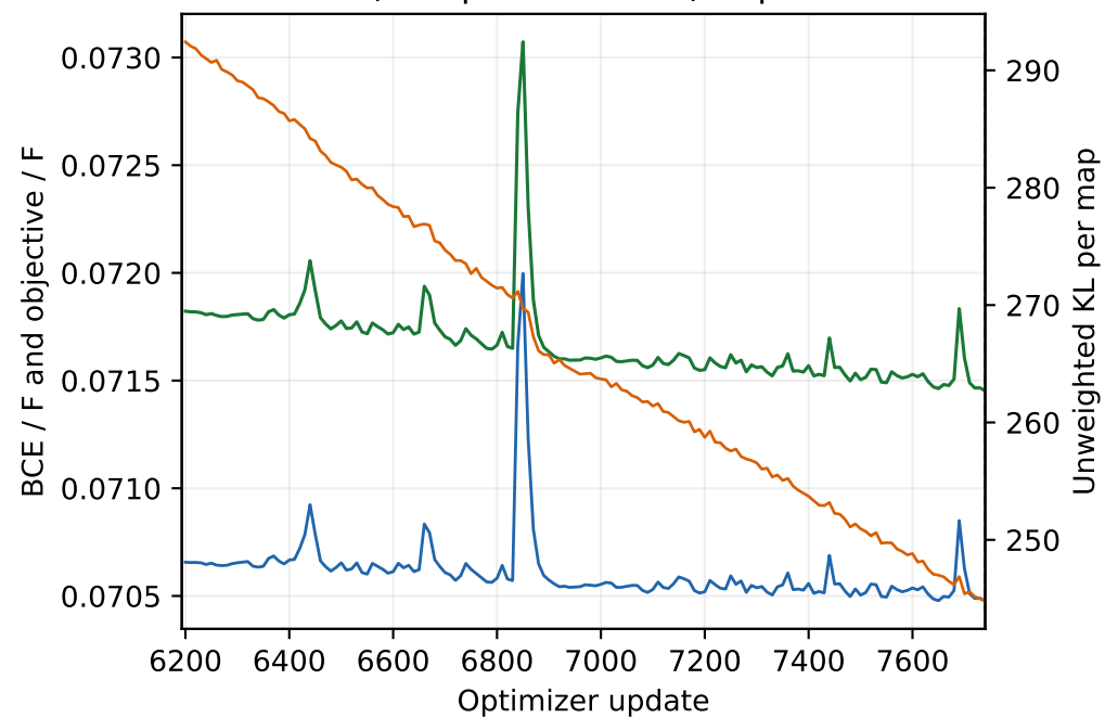
Stochastic train (10-update means) · updates 6193-7740
