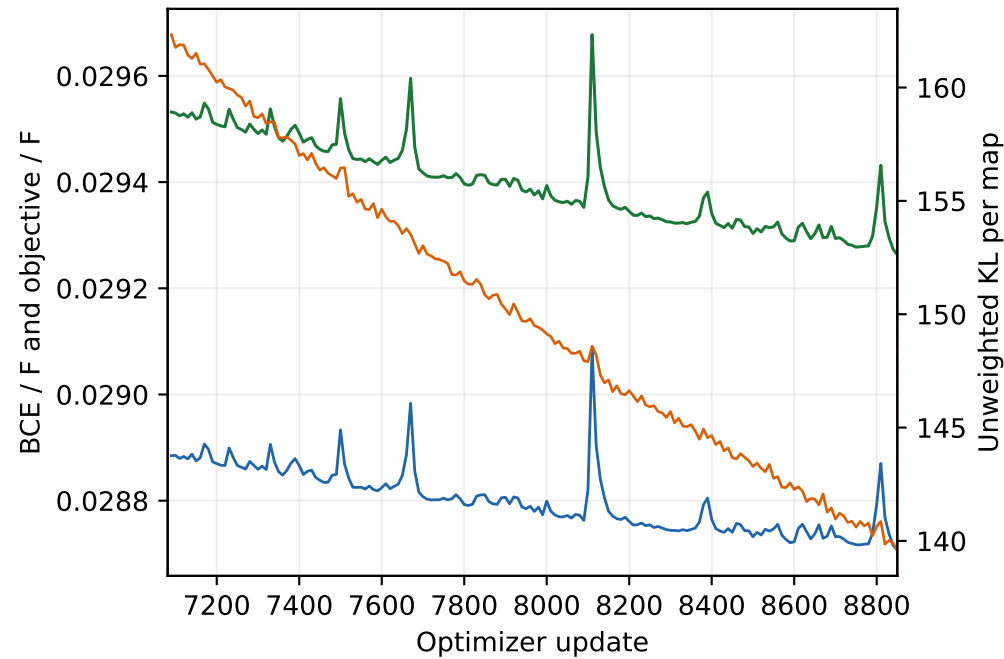
Stochastic train (10-update means) · updates 7081-8850
