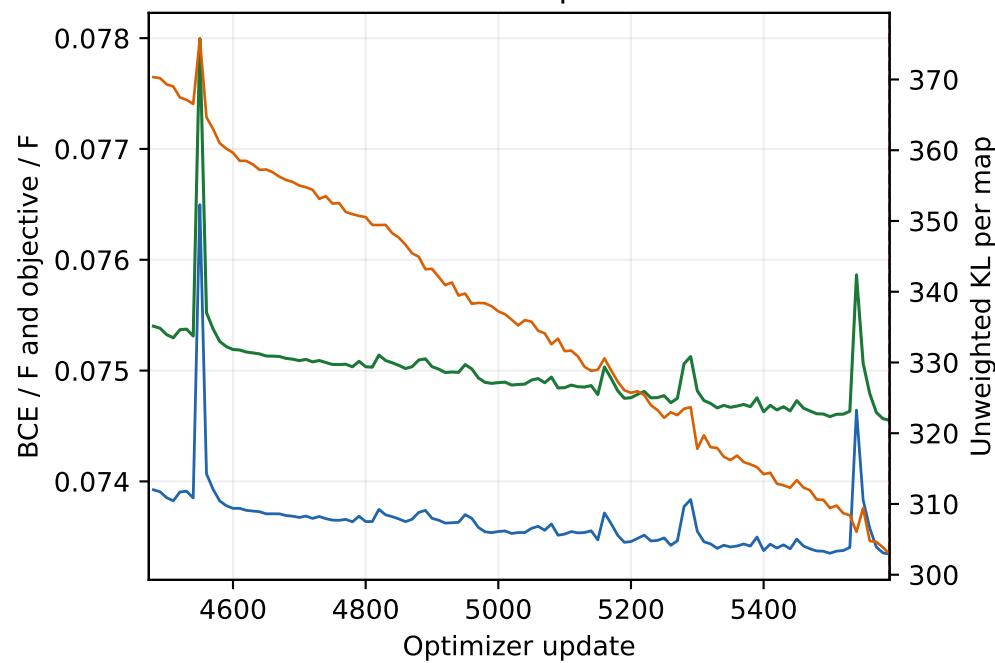
Posterior-mean train · updates 4473-5590
