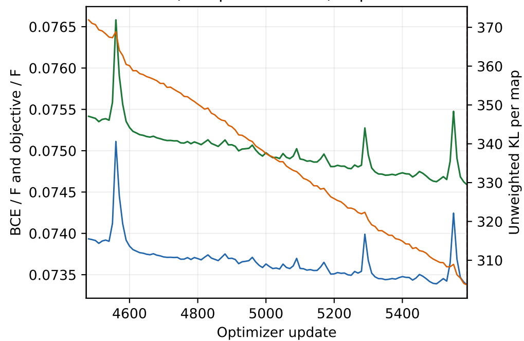
Stochastic train (10-update means) · updates 4473-5590
