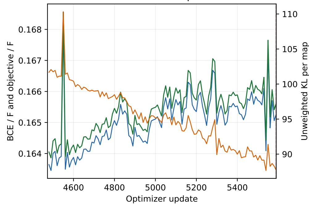
Posterior-mean validation · updates 4473-5590
