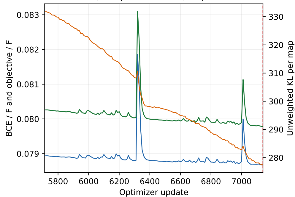
Stochastic train (10-update means) · updates 5713-7140
