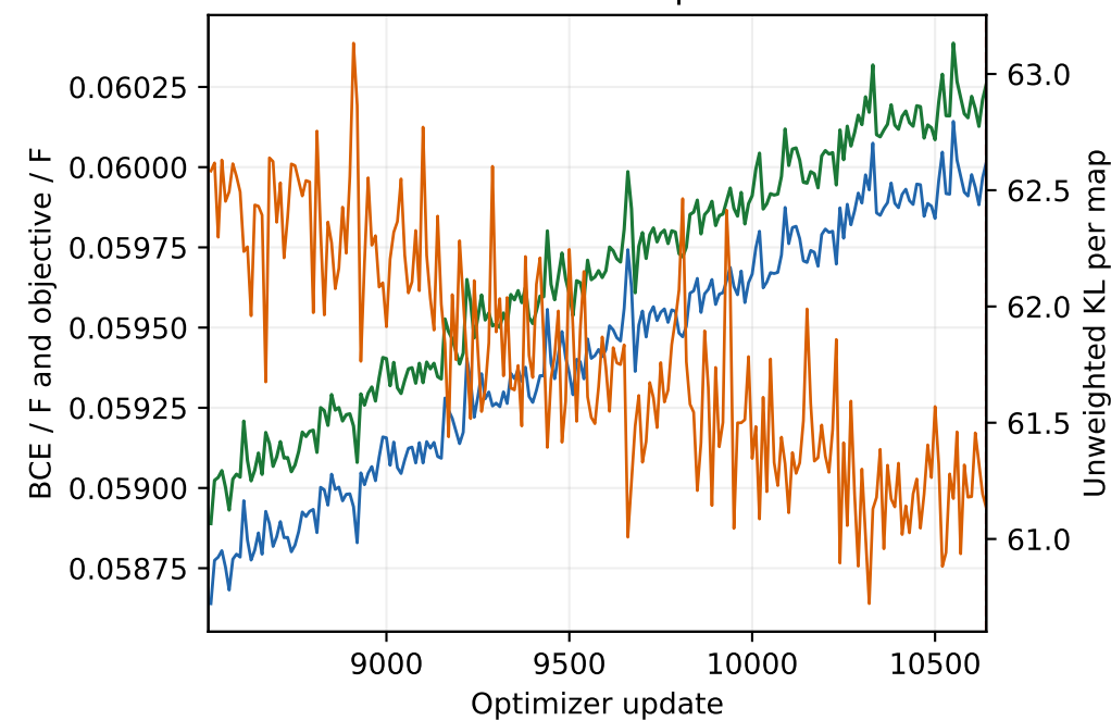
Posterior-mean validation · updates 8513-10640
