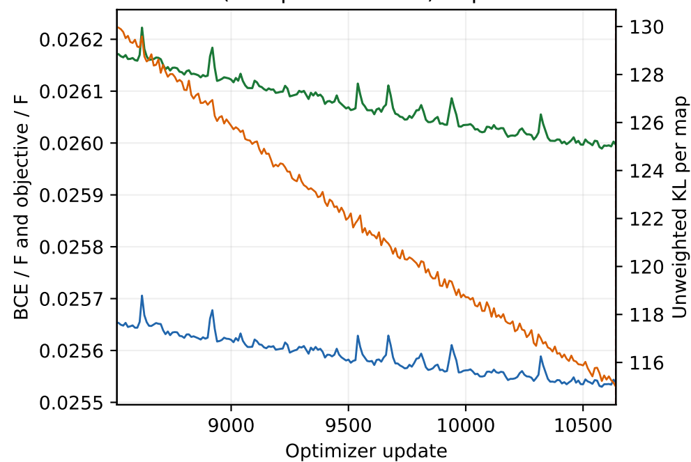
Stochastic train (10-update means) · updates 8513-10640
