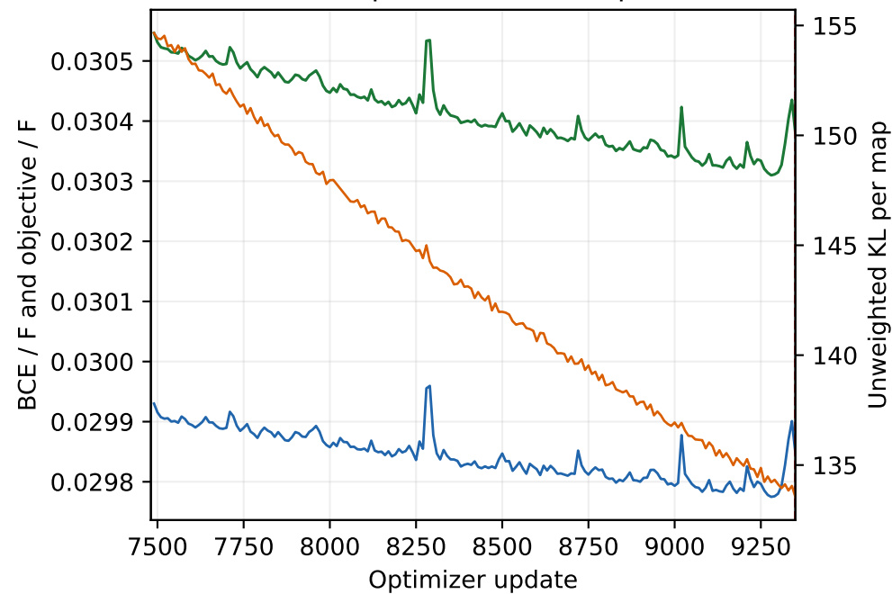
Stochastic train (10-update means) · updates 7481-9350
