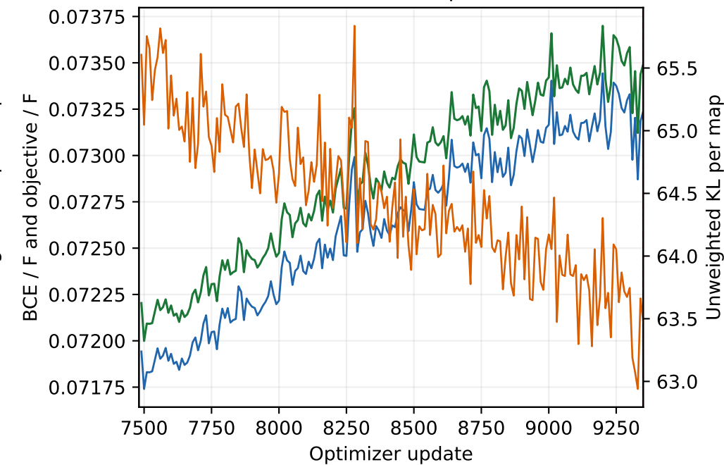
Posterior-mean validation · updates 7481-9350
