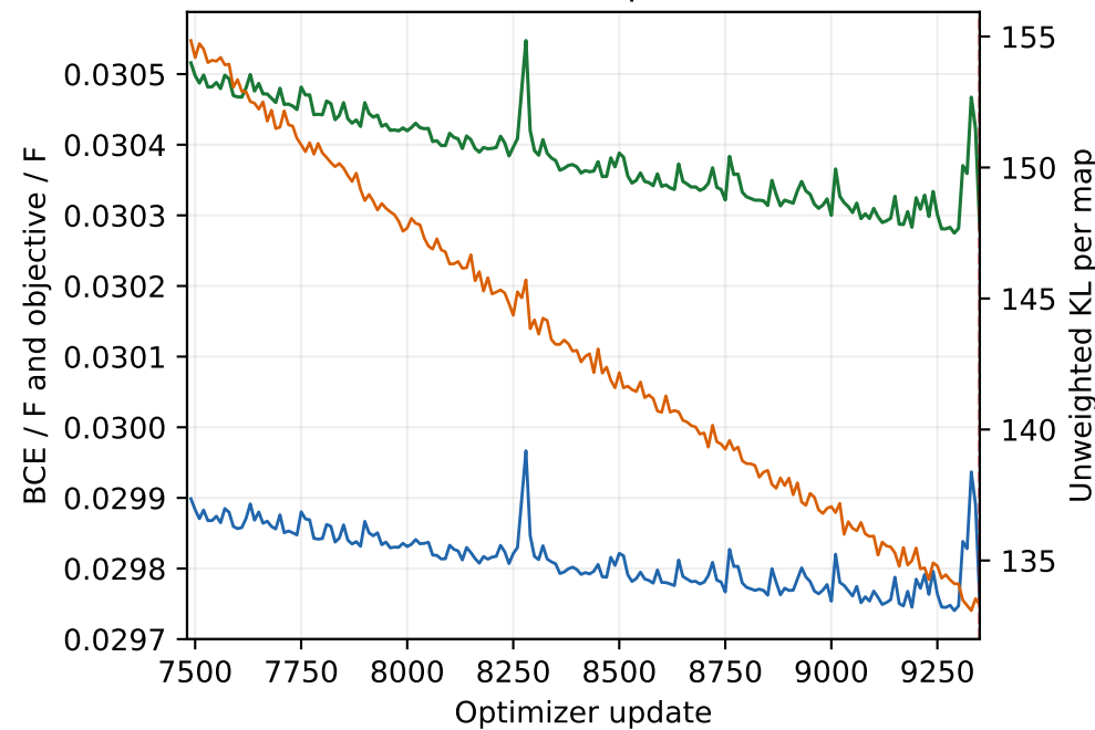
Posterior-mean train · updates 7481-9350
