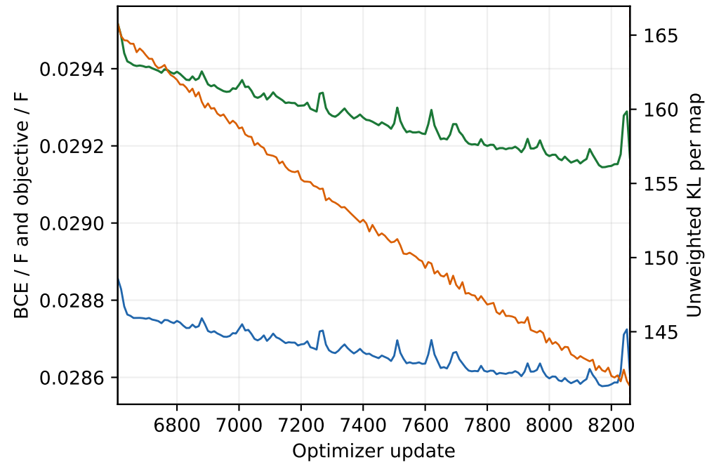
Stochastic train (10-update means) · updates 6609-8260
