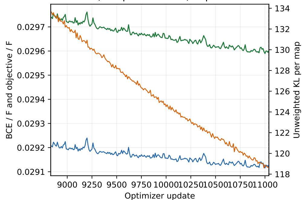
Stochastic train (10-update means) · updates 8833-11040
