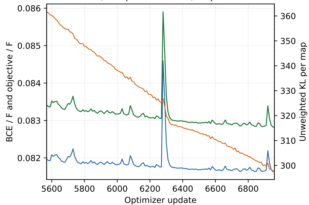
Stochastic train (10-update means) · updates 5569-6960
