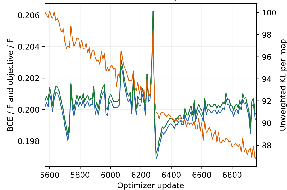
Posterior-mean validation · updates 5569-6960
