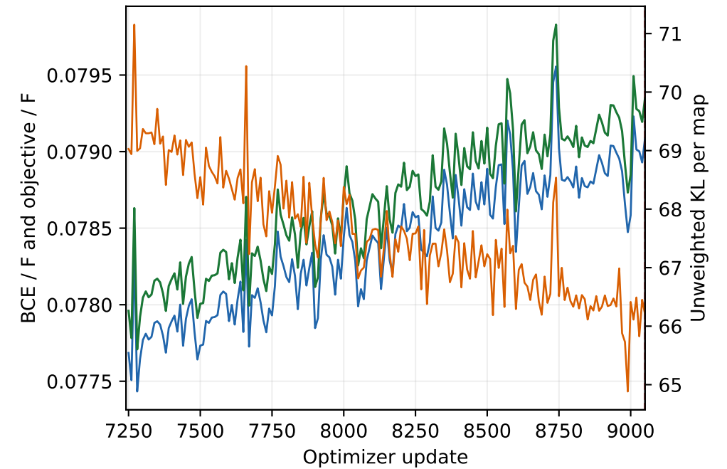
Posterior-mean validation · updates 7241-9050
