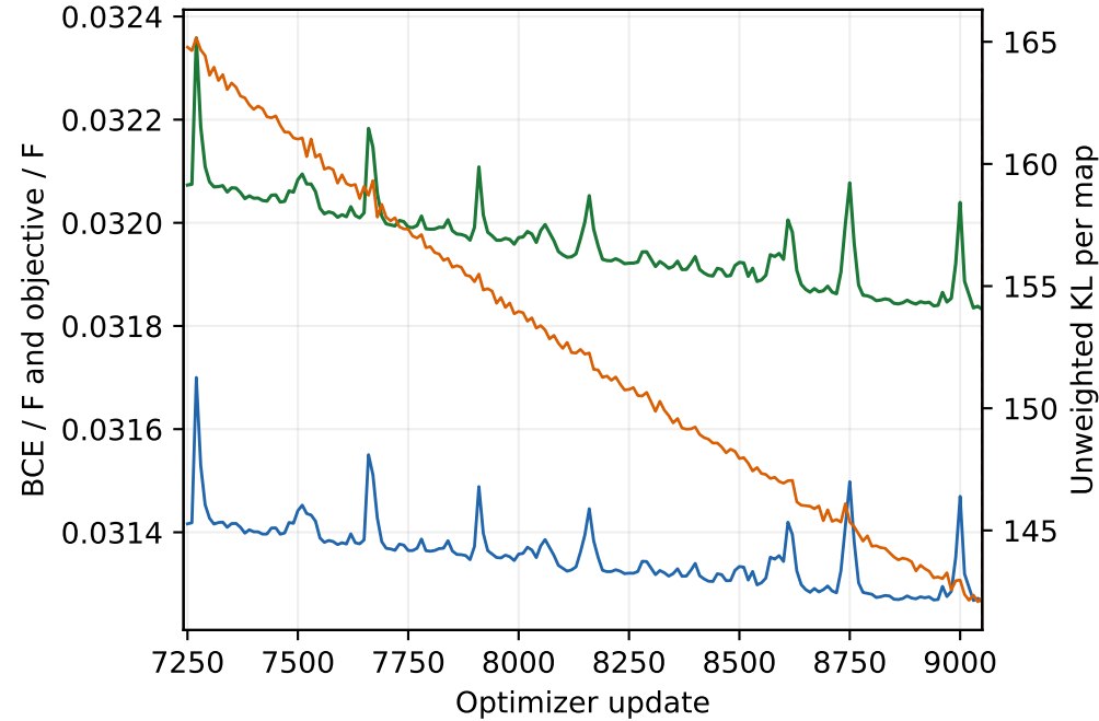
Stochastic train (10-update means) · updates 7241-9050
