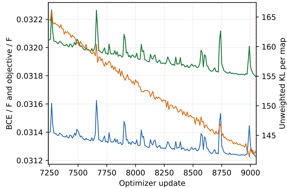
Posterior-mean train · updates 7241-9050
