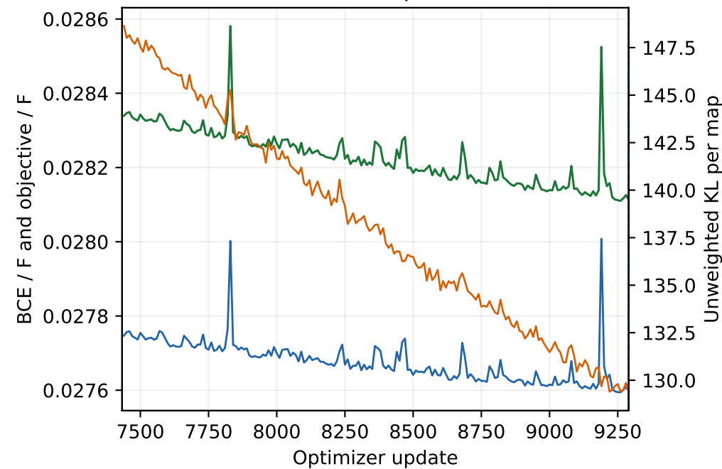
Posterior-mean train · updates 7433-9290
