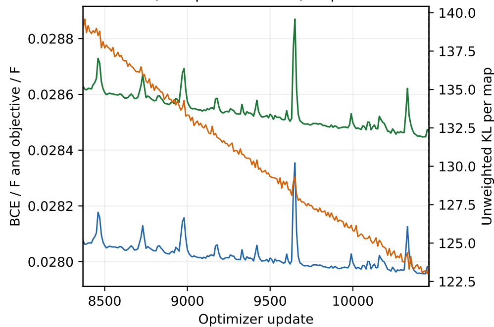
Stochastic train (10-update means) · updates 8369-10460
