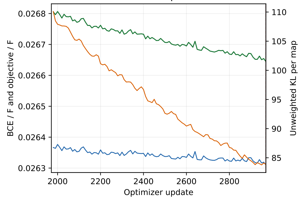
Posterior-mean train · updates 1971-2970
