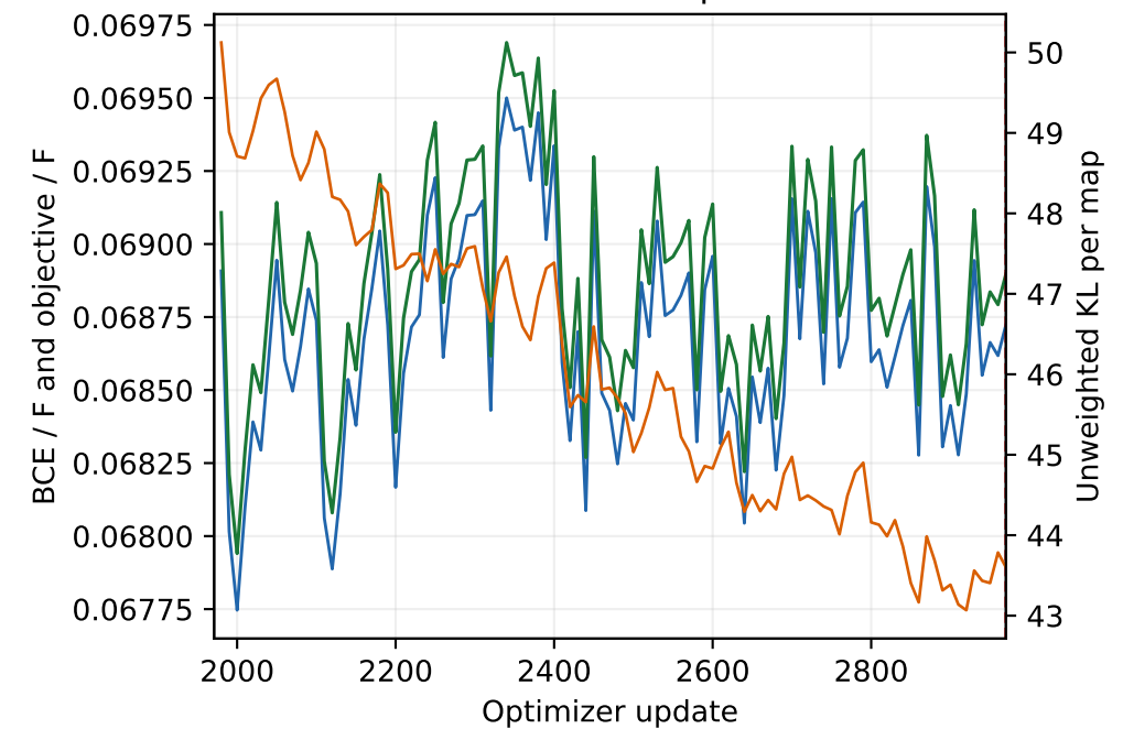
Posterior-mean validation · updates 1971-2970
