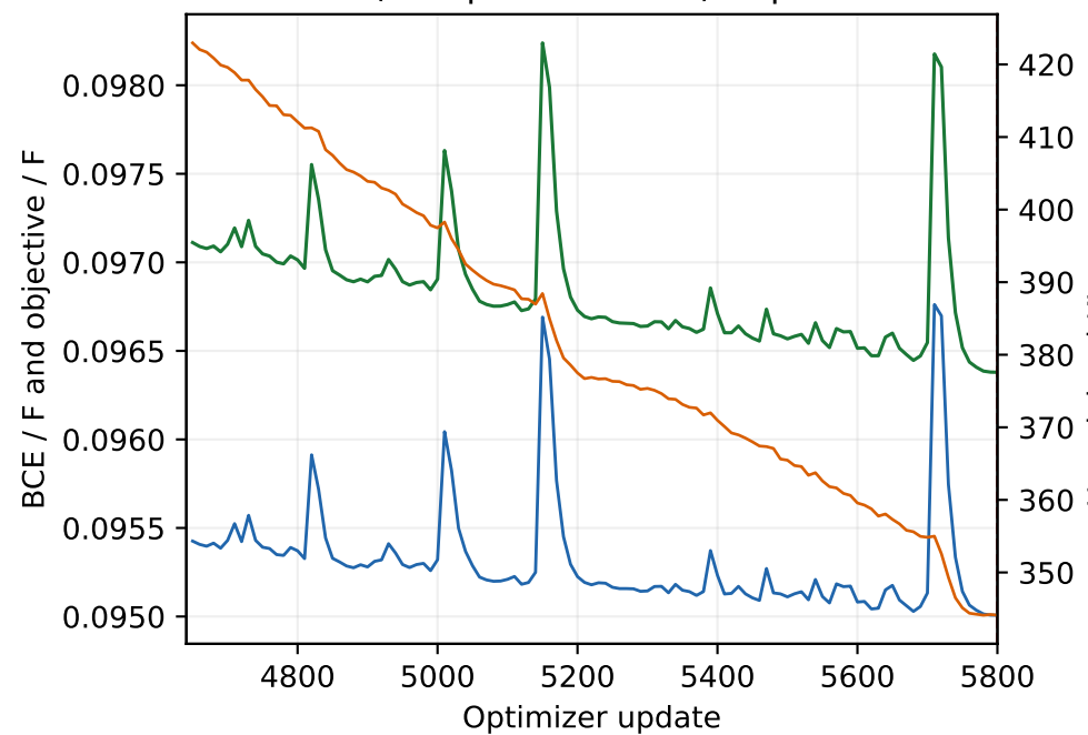
Stochastic train (10-update means) · updates 4641-5800
