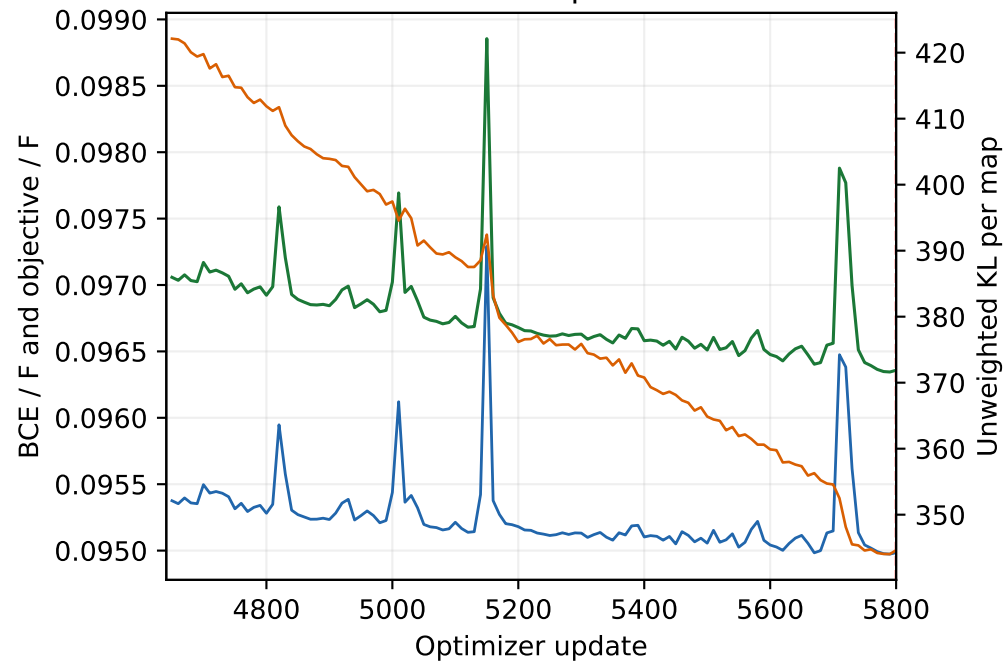
Posterior-mean train · updates 4641-5800
