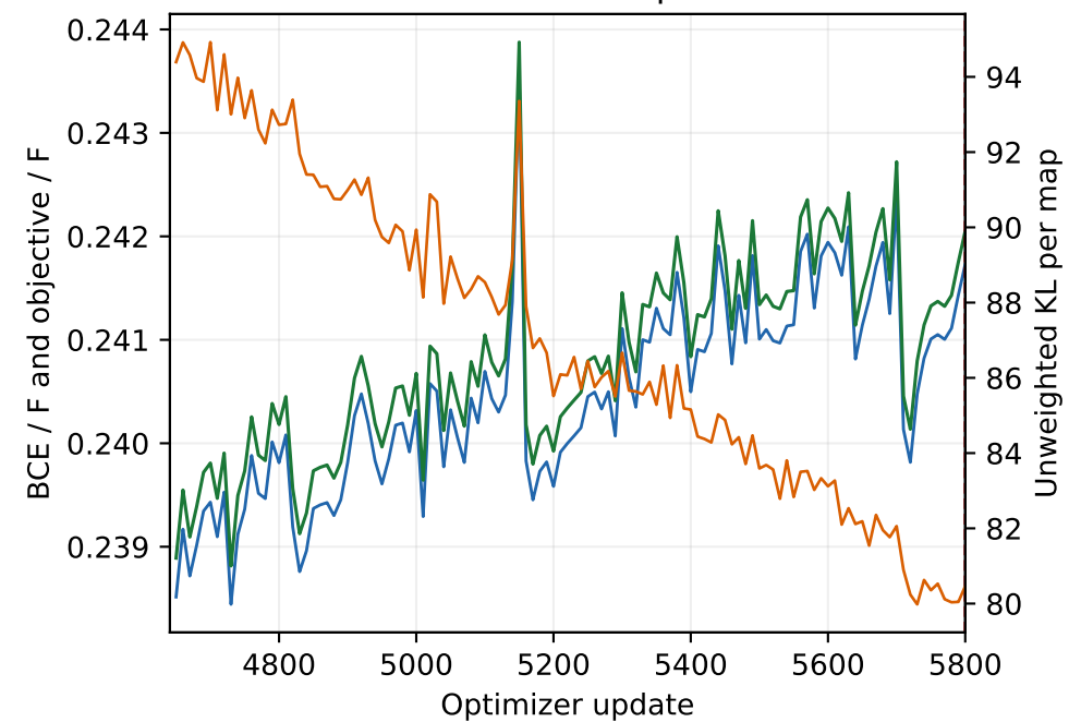
Posterior-mean validation · updates 4641-5800
