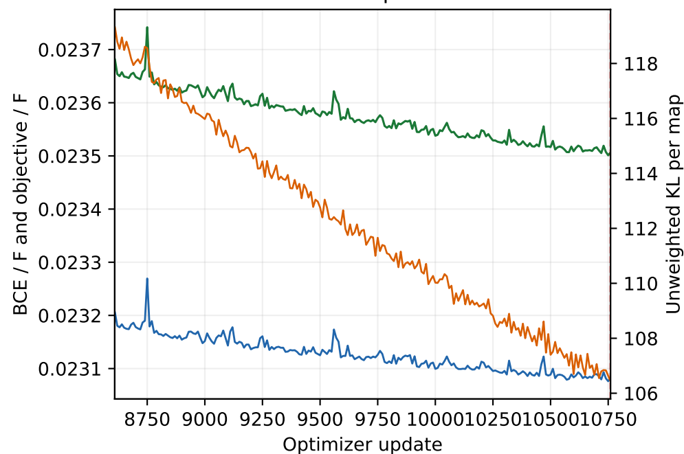
Posterior-mean train · updates 8609-10760
