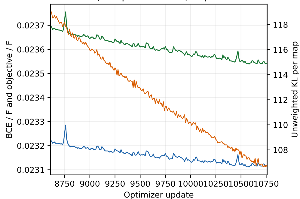
Stochastic train (10-update means) · updates 8609-10760
