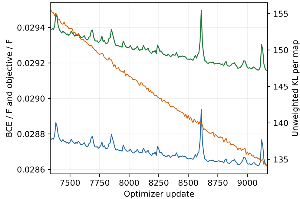
Stochastic train (10-update means) · updates 7337-9170
