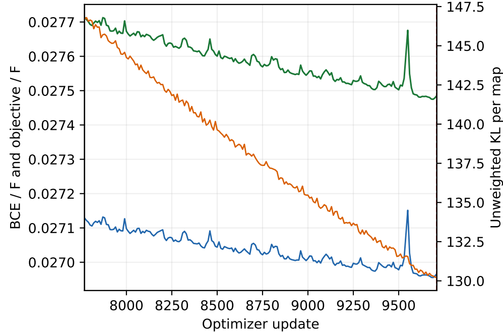
Stochastic train (10-update means) · updates 7769-9710
