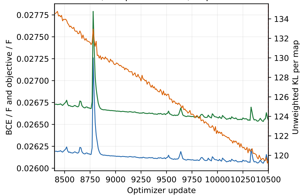
Stochastic train (10-update means) · updates 8401-10500
