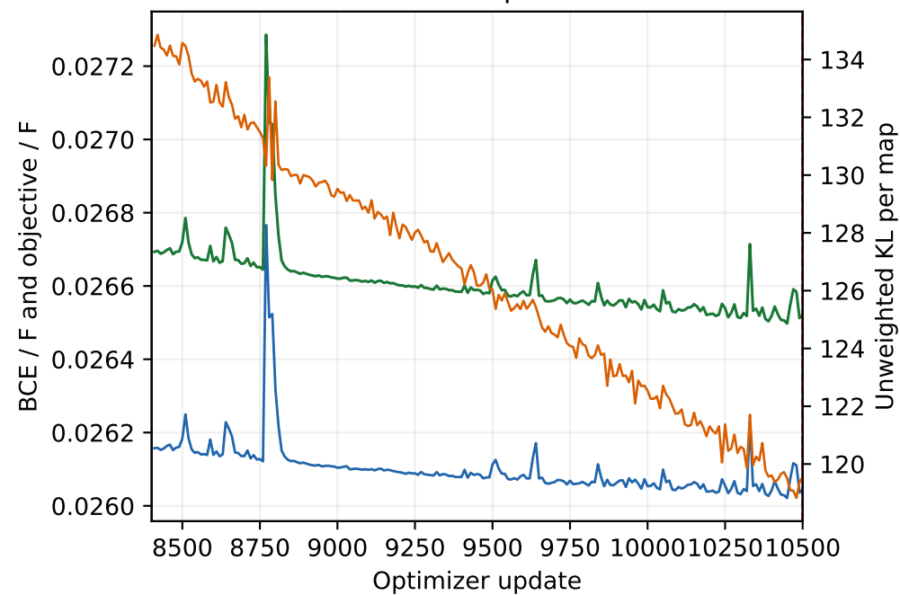
Posterior-mean train · updates 8401-10500
