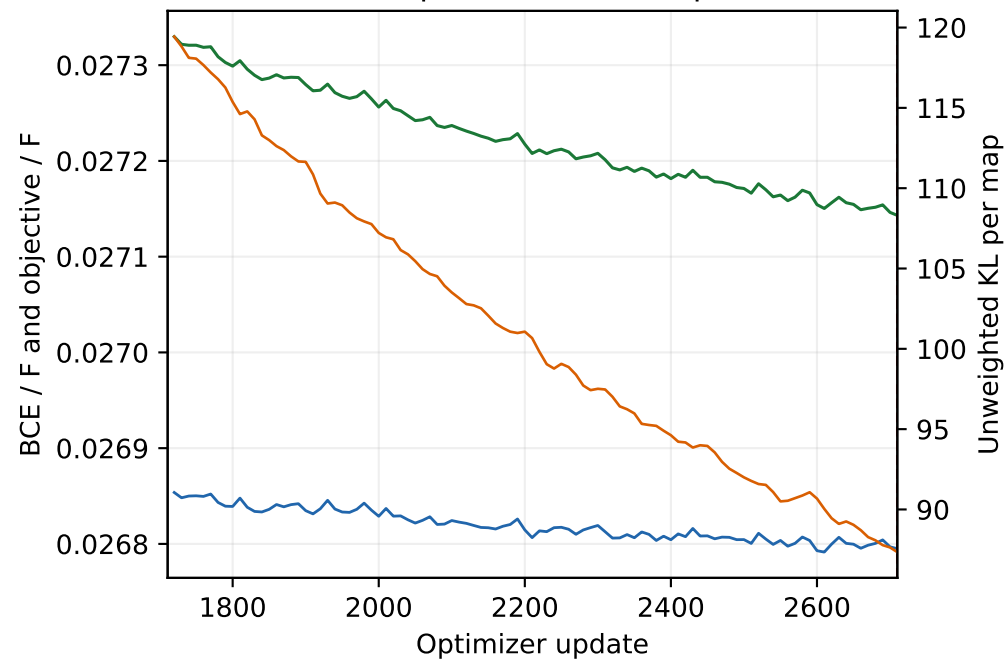
Stochastic train (10-update means) · updates 1711-2710
