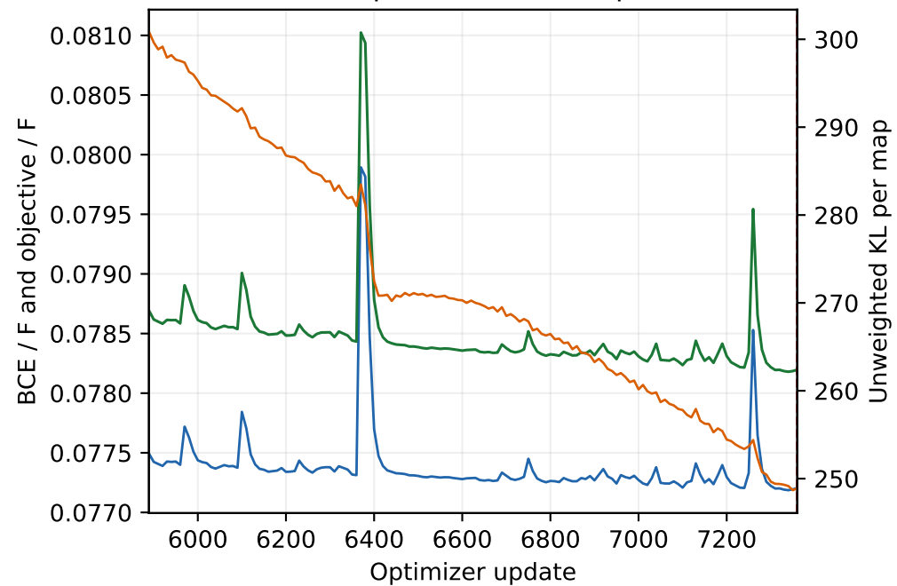
Stochastic train (10-update means) · updates 5889–7360
