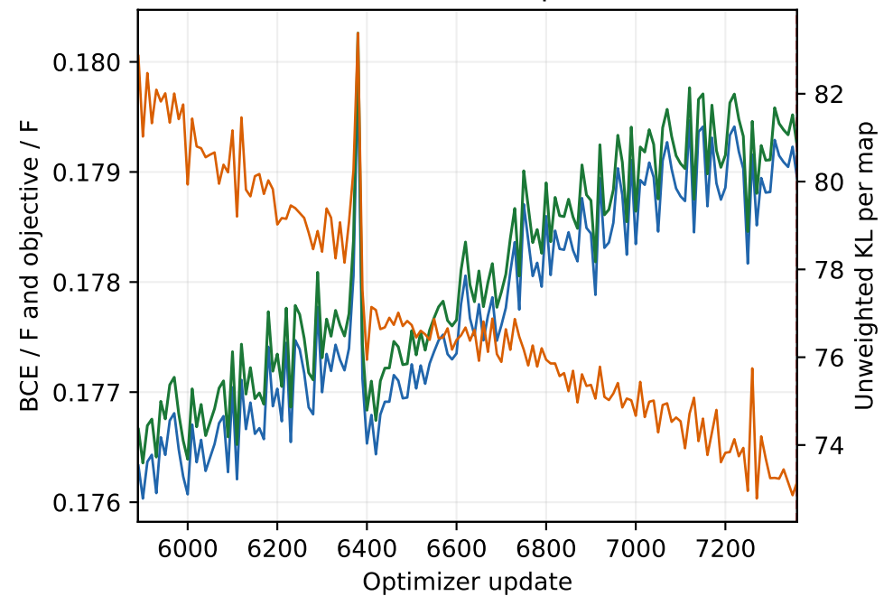
Posterior-mean validation · updates 5889–7360
