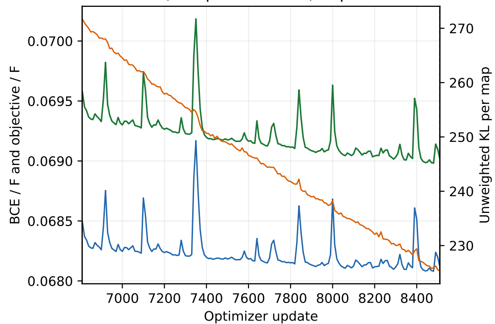
Stochastic train (10-update means) · updates 6809-8510
