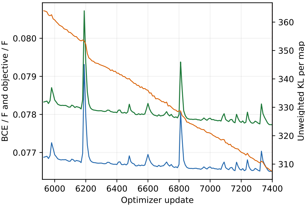
Stochastic train (10-update means) · updates 5921-7400
