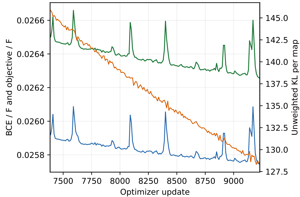
Stochastic train (10-update means) · updates 7385-9230
