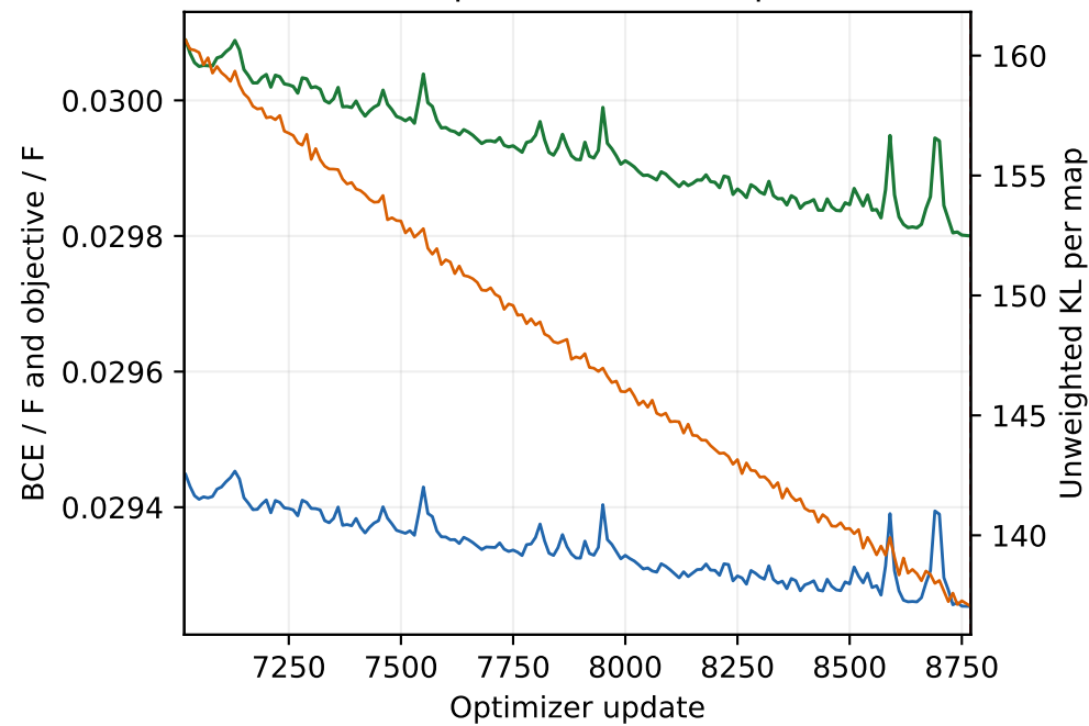
Stochastic train (10-update means) · updates 7017-8770
