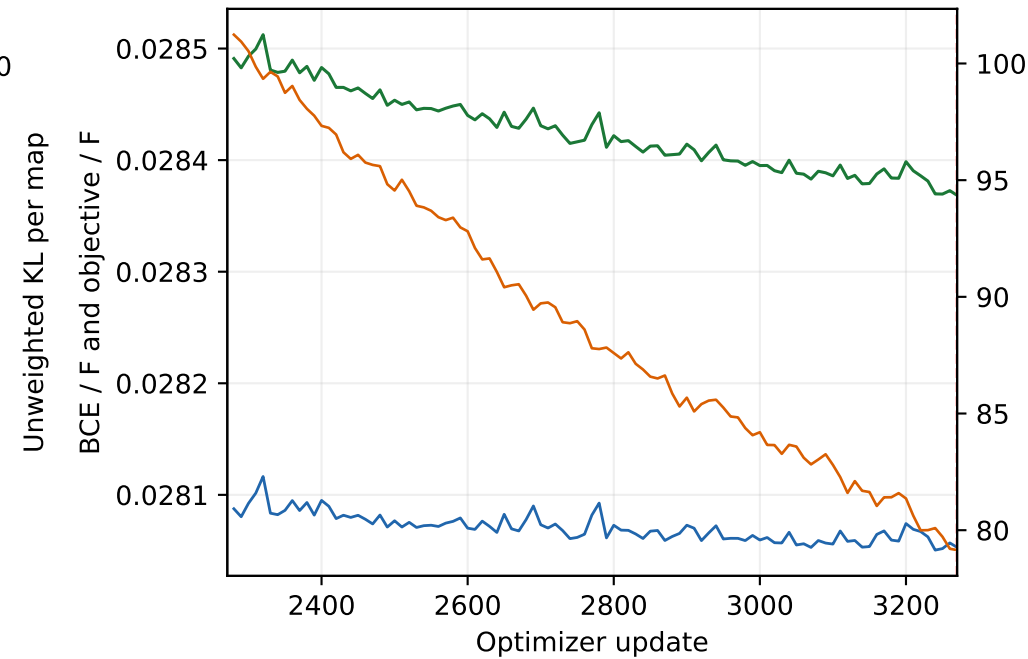
Posterior-mean train · updates 2271-3270
