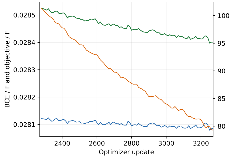
Stochastic train (10-update means) · updates 2271-3270
