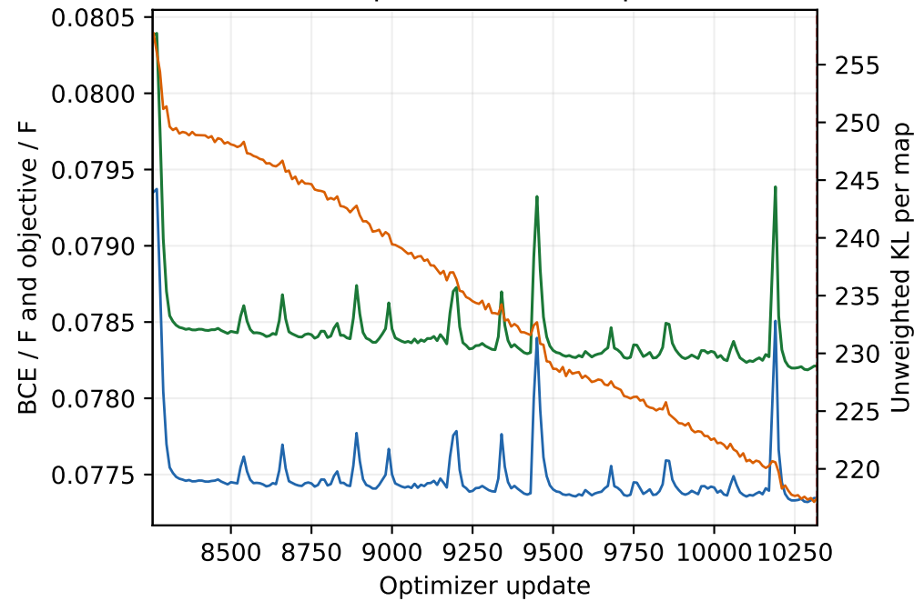
Stochastic train (10-update means) · updates 8257-10320
