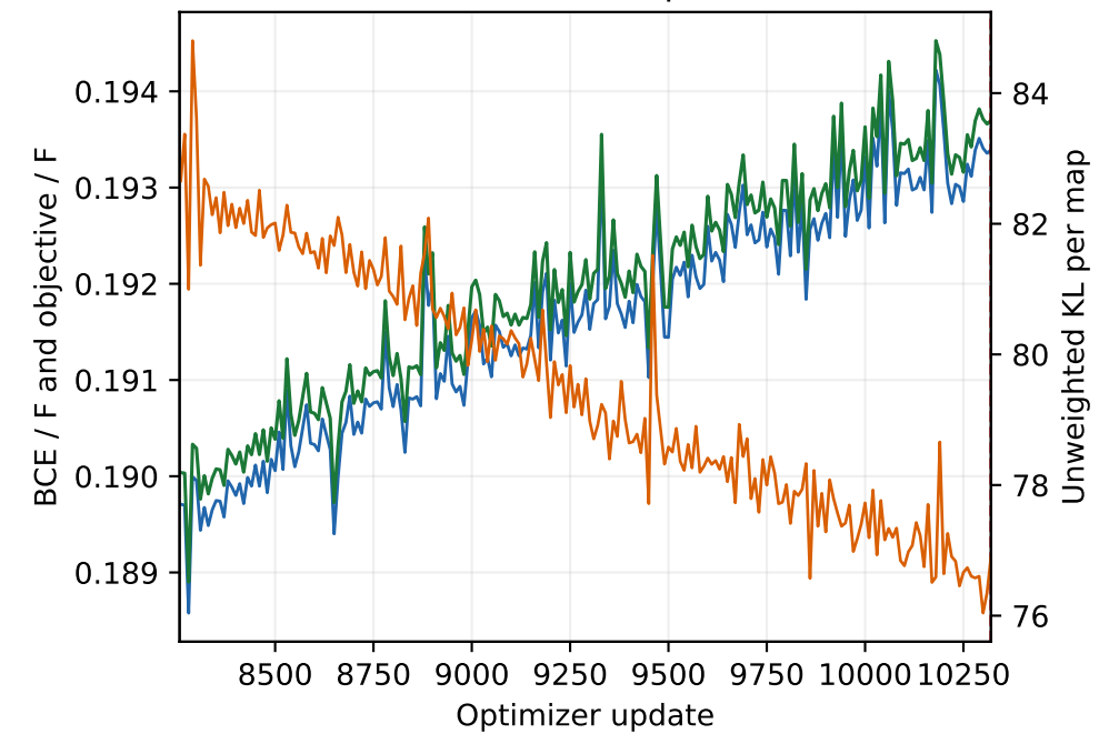
Posterior-mean validation · updates 8257-10320
