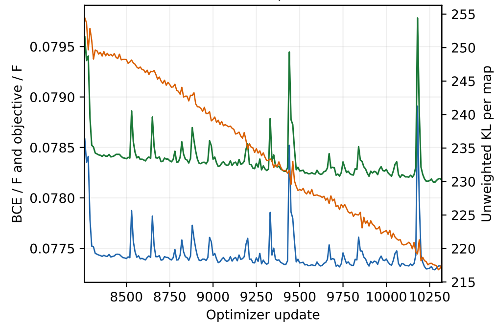
Posterior-mean train · updates 8257-10320
