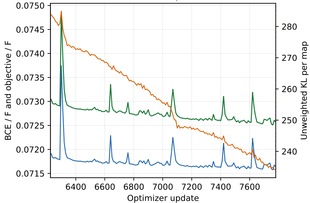
Posterior-mean train · updates 6225-7780
