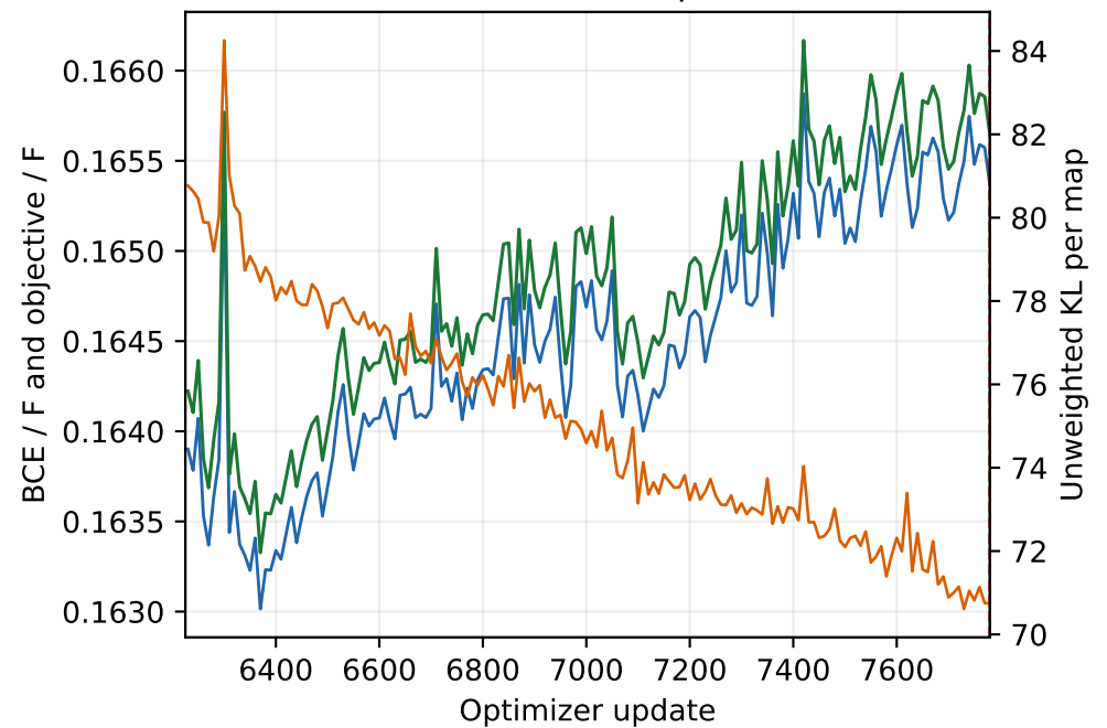
Posterior-mean validation · updates 6225-7780
