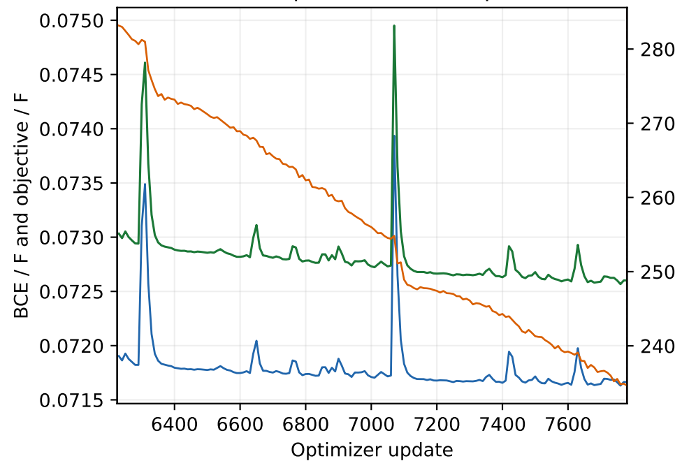
Stochastic train (10-update means) · updates 6225-7780
