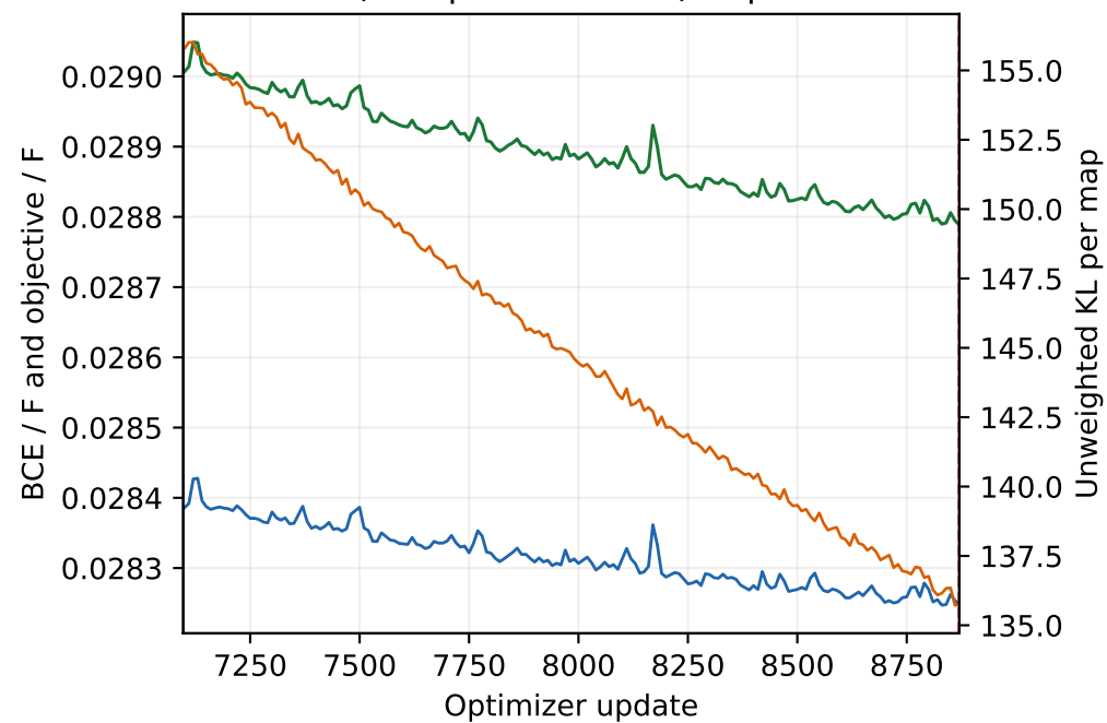
Stochastic train (10-update means) · updates 7097-8870
