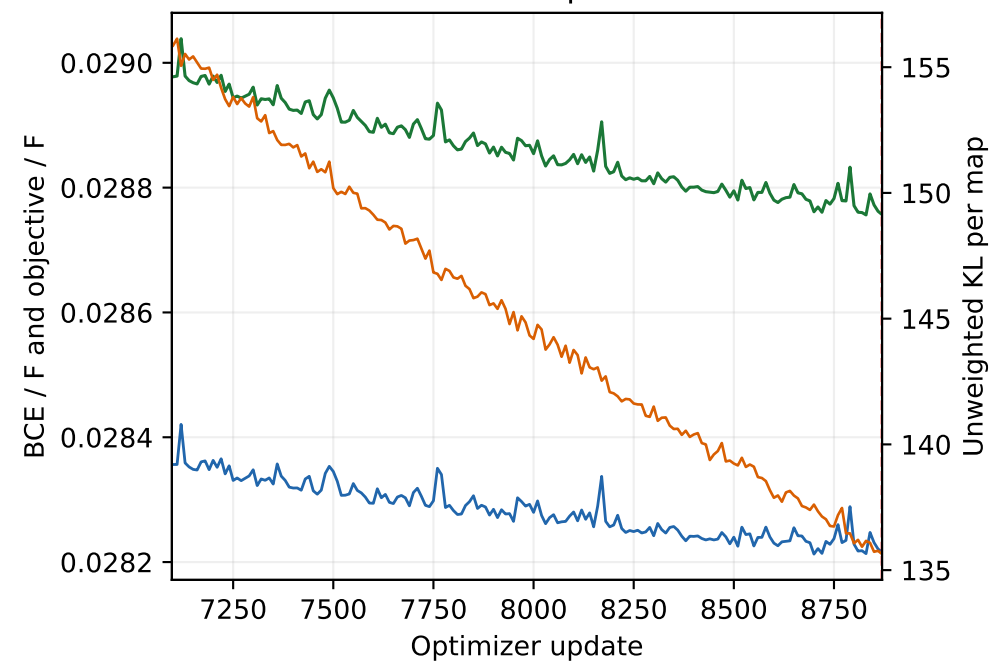
Posterior-mean train · updates 7097-8870
