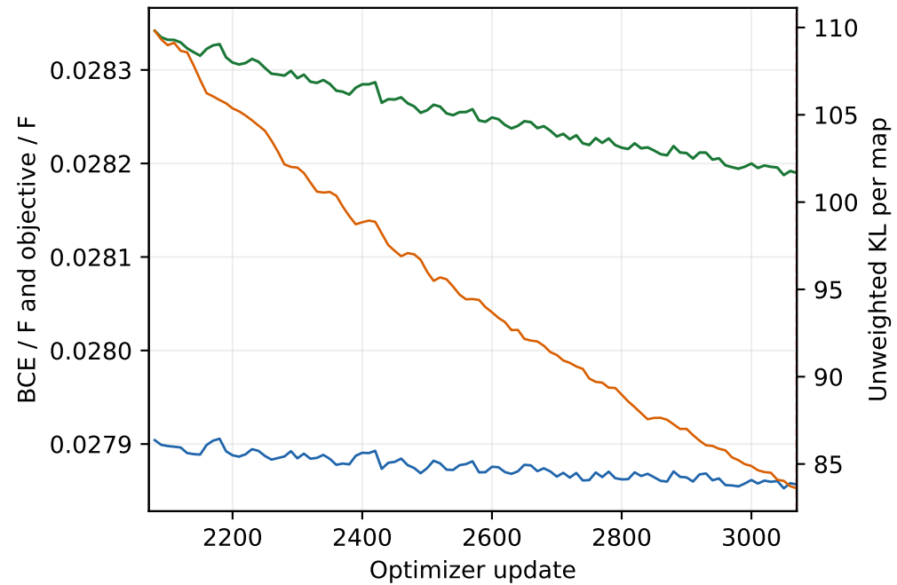
Stochastic train (10-update means) · updates 2071-3070
