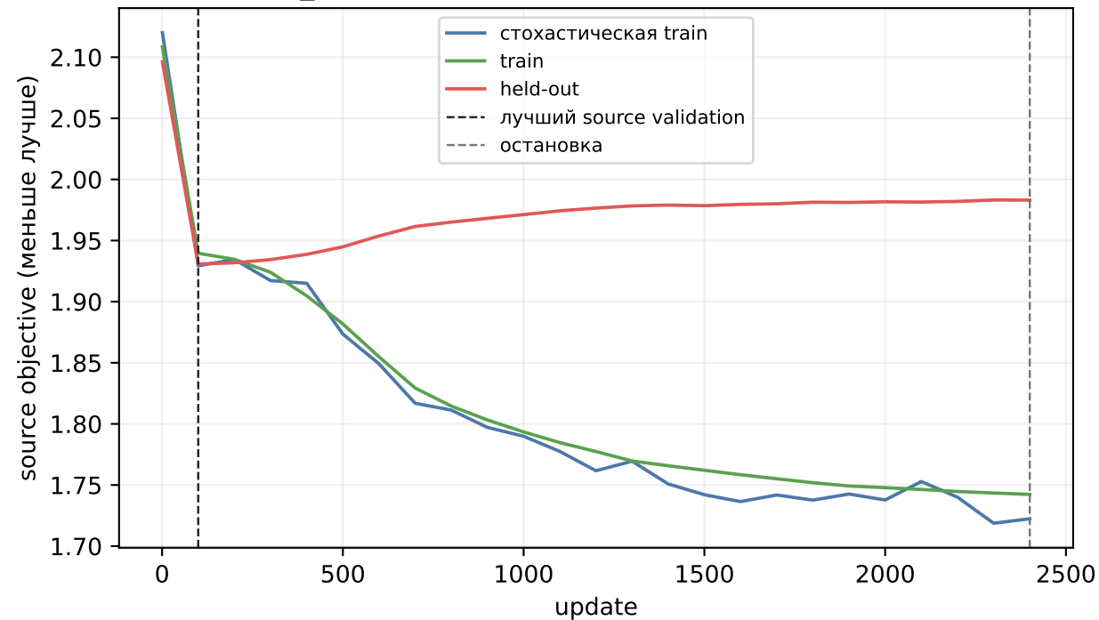
flow_matching, seed 4100: source-only обучение
