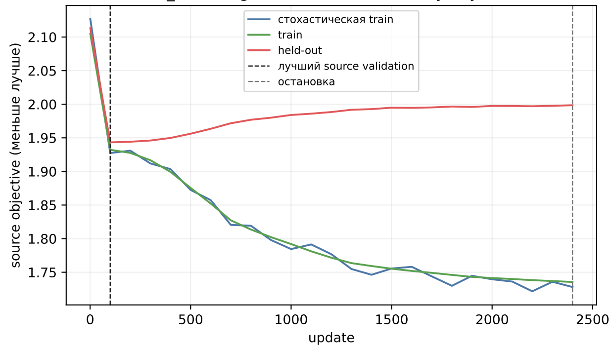
flow_matching, seed 4104: source-only обучение
