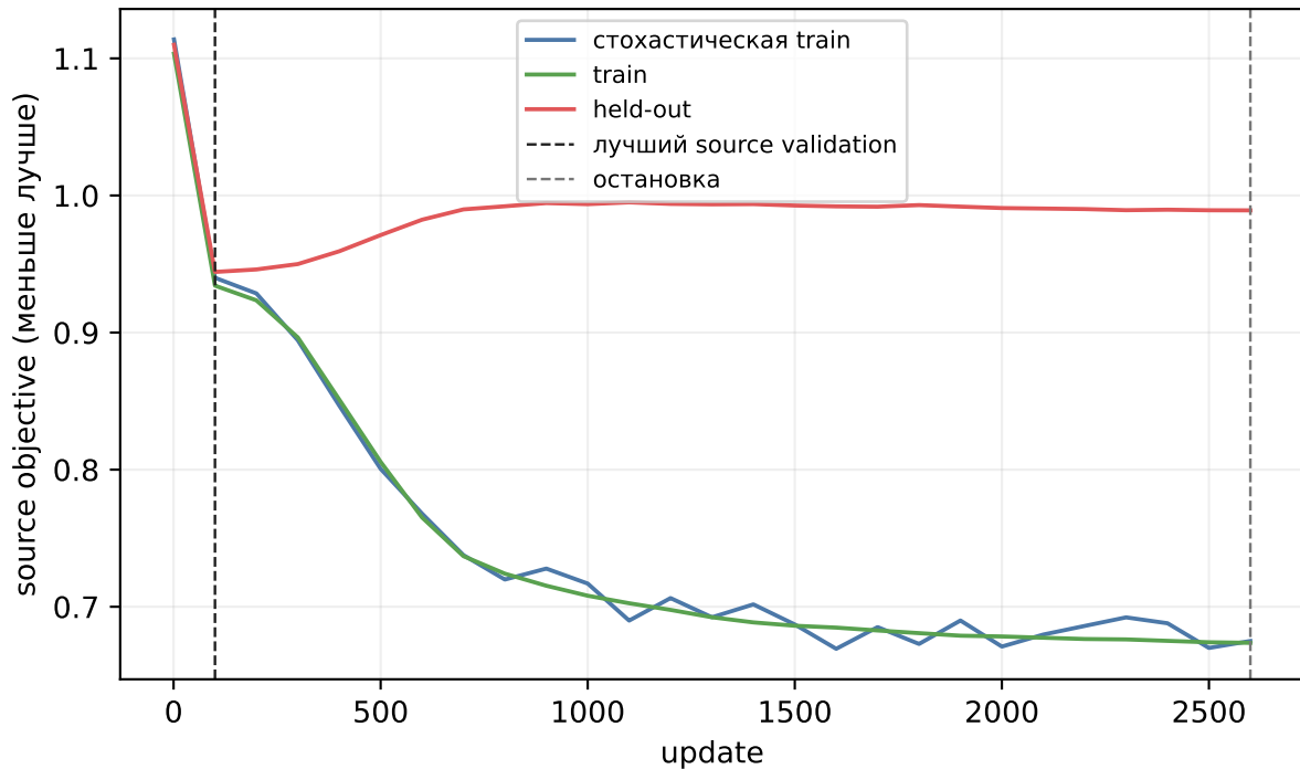
diffusion, seed 4106: source-only обучение
