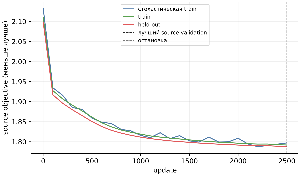
set_transformer_flow, seed 4100: source-only обучение
