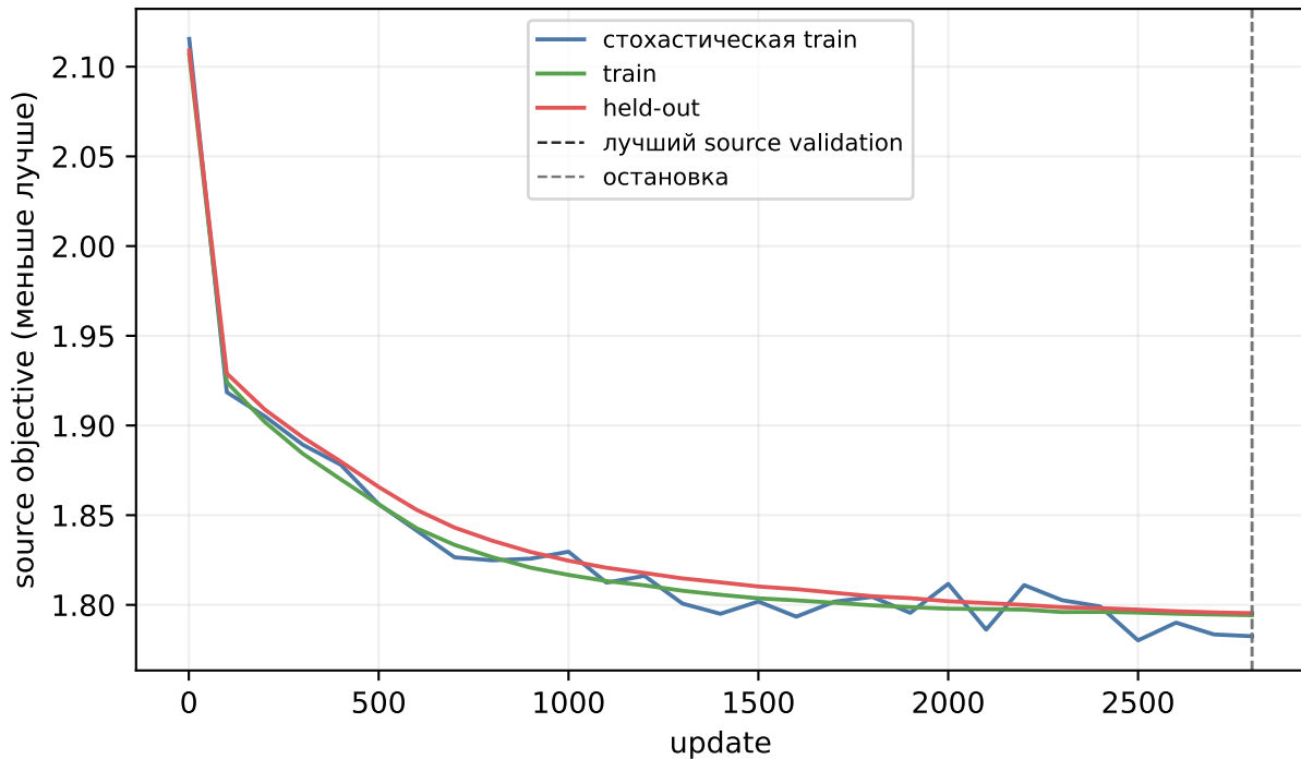
set_transformer_flow, seed 4101: source-only обучение
