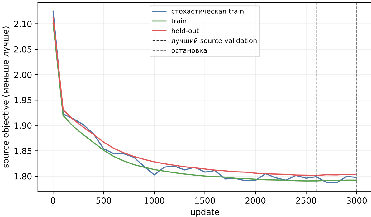
set_transformer_flow, seed 4102: source-only обучение
