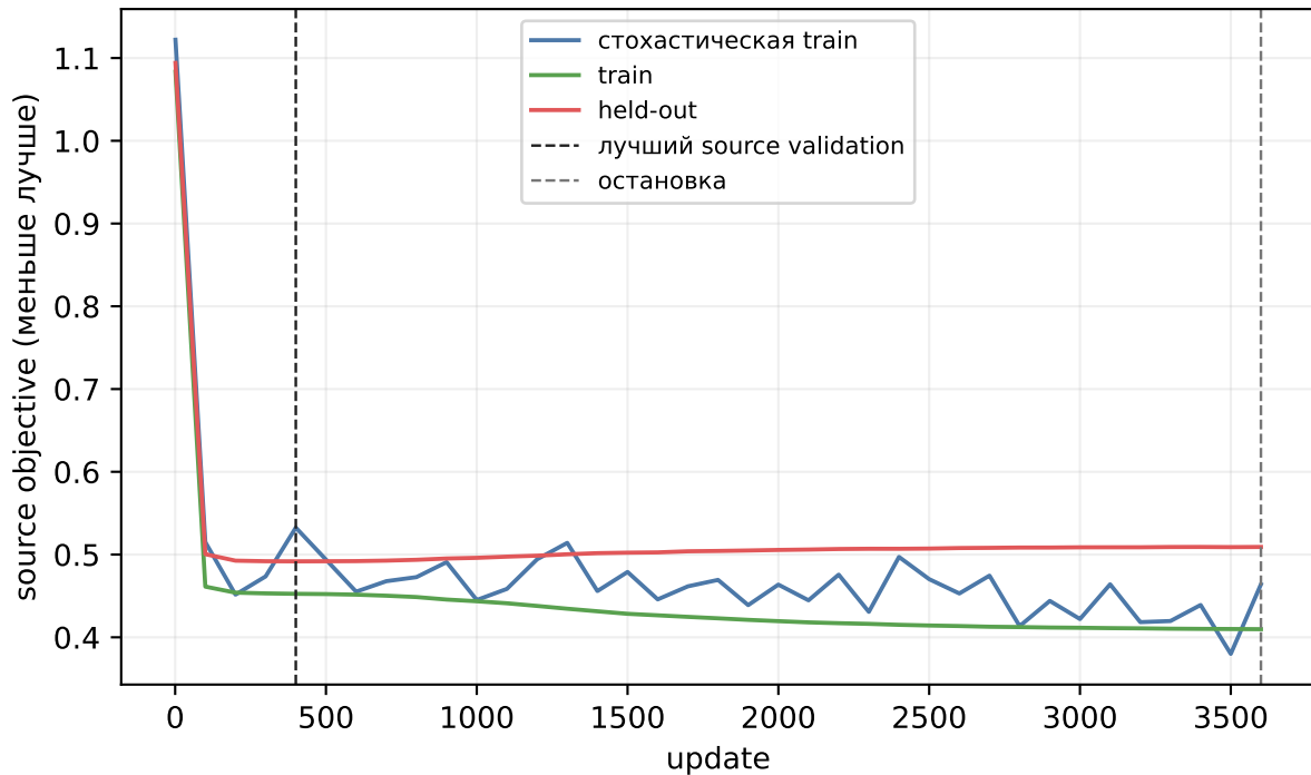
diffusion, seed 4103: source-only обучение
