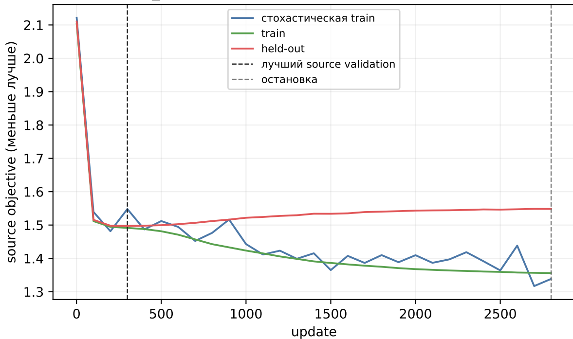
flow_matching, seed 4103: source-only обучение
